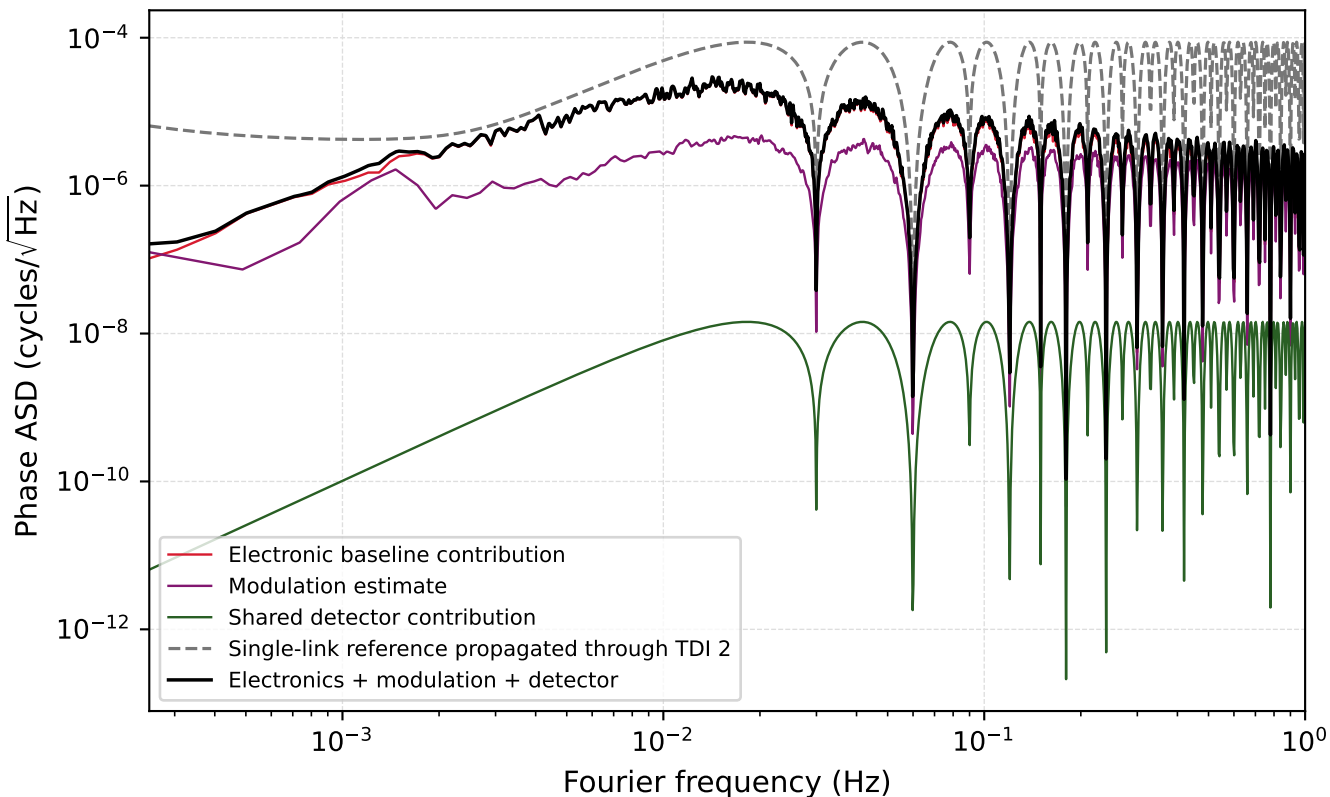
Varying-arm TDI 2 + clock correction; component estimate
