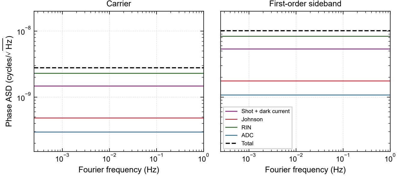
FIG. 5. Predicted Newport carrier and first-order sideband readout noise for one modulated and one unmodulated beam, each delivering 8mW at the detector, with modulation depth 0.53rad. The two panels share a common vertical scale. Shot noise includes dark-current shot noise; the ADC contribution is the white quantization estimate. The dashed curves are the quadrature totals. The different beat amplitudes in Eq. (??) give different carrier and sideband phase-noise levels even though their input current-noise spectra are taken to be equal.
