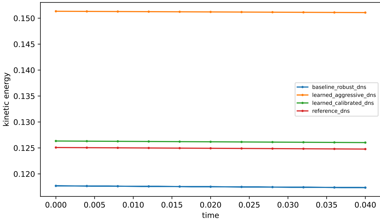
3D Navier--Stokes: kinetic-energy decay
