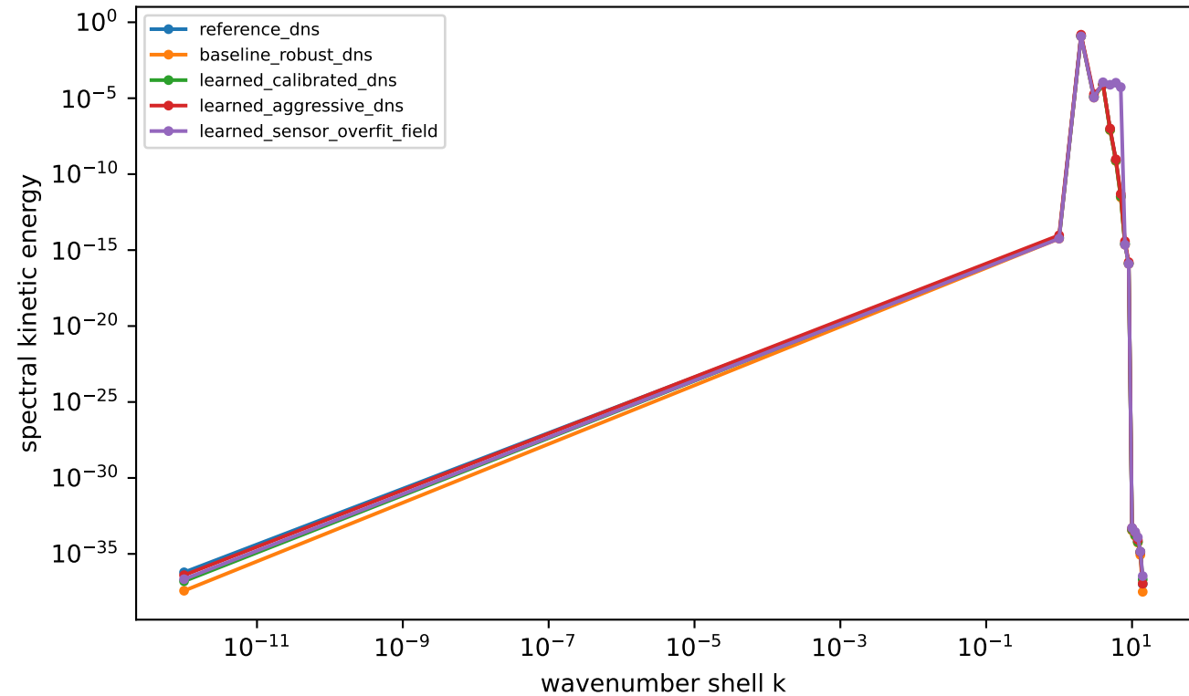
Final 3D kinetic-energy spectra
