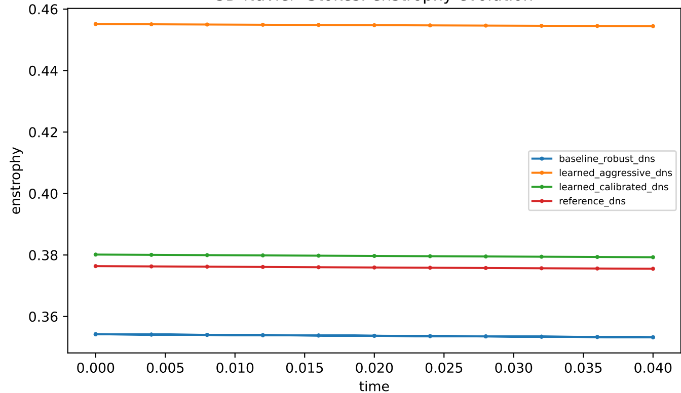
3D Navier--Stokes: enstrophy evolution
