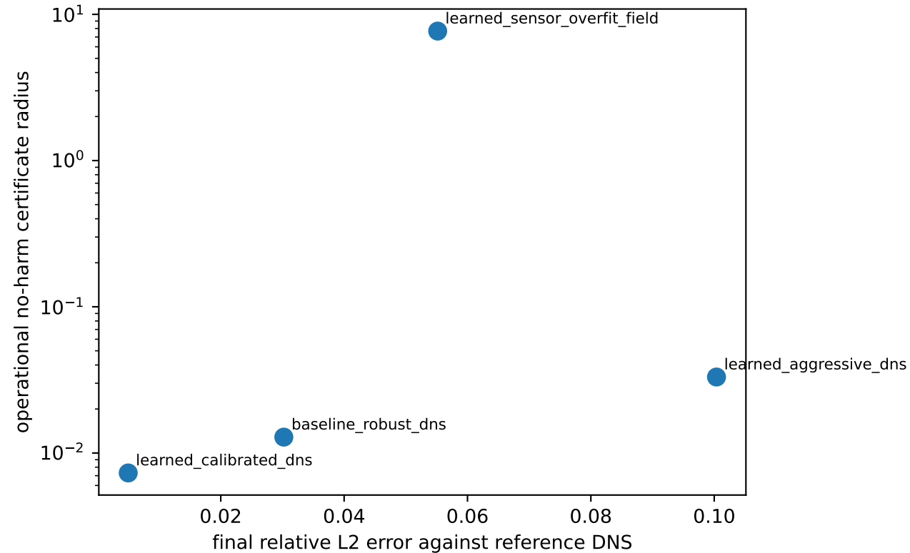
No-harm NS3D: error versus certificate radius
