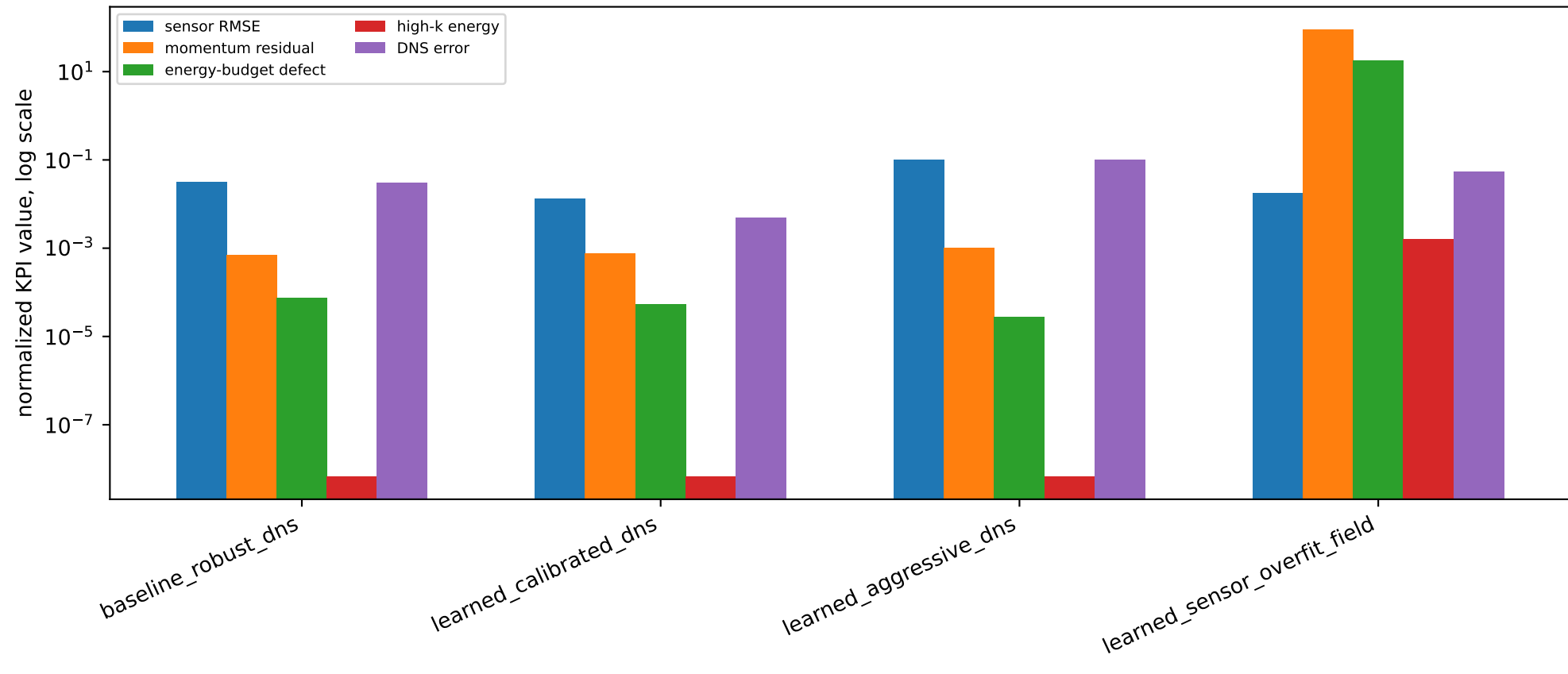
Industrial no-harm KPIs for 3D Navier--Stokes candidates
