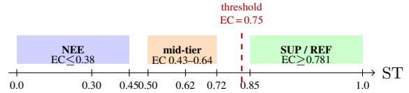
Figure 2: Trust tiers on the benchmark. Evidence text is byte-identical across all tiers; only the ST scalar changes. The red dashed line marks the EC = 0.75 decision threshold; all high-trust records ( ST \geq 0.85 , EC \geq 0.781 ) clear it. Mid-tier probes ( EC \in \{0.43-0.64\} ) fall below it, testing whether a model reasons continuously rather than thresholds ST into two bins.
