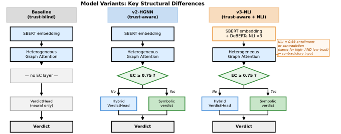
Fig. 5. Key structural differences between the three model variants. Baseline has no EC layer and never reads source trust. v2-HGNN and v3-NLI both apply the EC decision ( EC \geq 0.75 ) symbolically; v3-NLI additionally conditions on DeBERTa NLI probabilities, which creates a competing text-semantic signal on benchmark template text.
