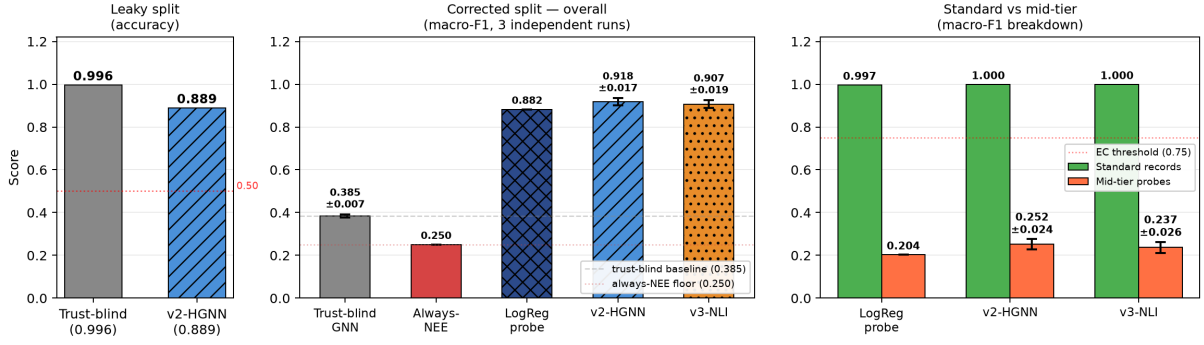
Figure 6: The inversion. On the original leaky split a trust-blind model wins on accuracy; on the corrected split it collapses to chance (macro-F1) while a trust-aware model wins, with both the controlled probe and the original graph network.
