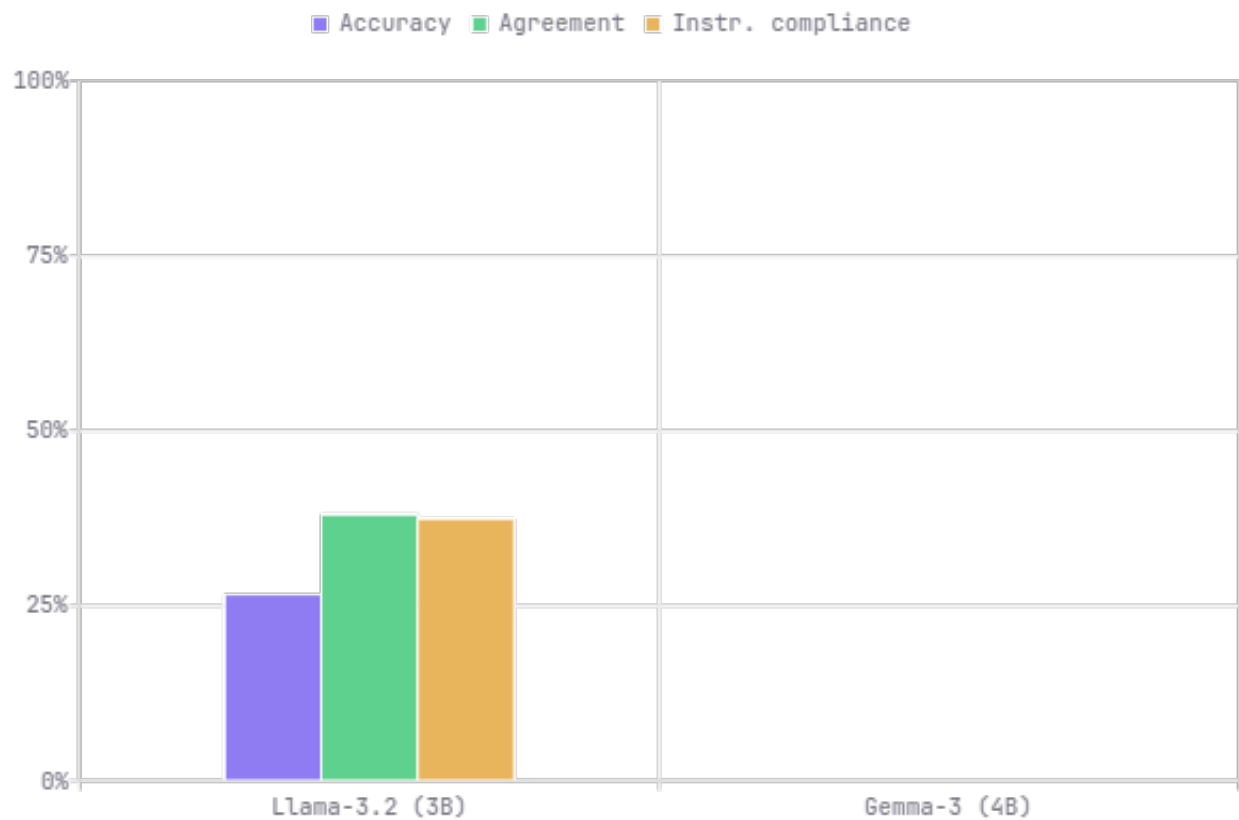
Accuracy, agreement & compliance – all locally benchmarked models
