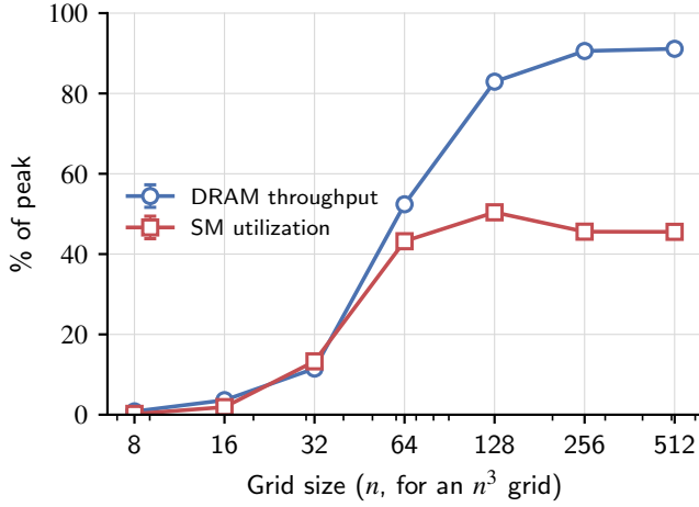
Fig. 5. Achieved DRAM throughput and SM utilization (% of peak) vs. grid size. DRAM throughput overtakes and pulls away from SM utilization beyond 64^3 cells.
