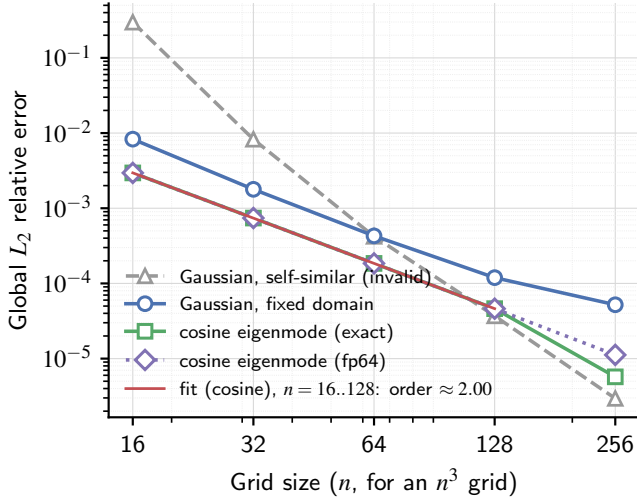
Fig. 1. Global L_2 relative error vs. grid size for the invalid self-similar sweep, the fixed-domain Gaussian sweep, and the exact cosine eigenmode (single and double precision), with the fitted order for the fp32 cosine. The Gaussian bends up at n = 256 (boundary-modeling floor); the fp32 cosine dips below the trend there (single-precision rounding), while the fp64 cosine continues the second-order trend, confirming that dip is an arithmetic artifact.
