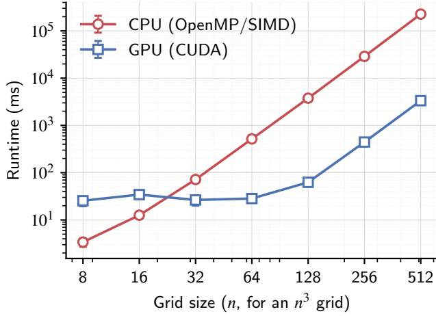
Fig. 2. Runtime vs. grid size for both backends (log-log).
