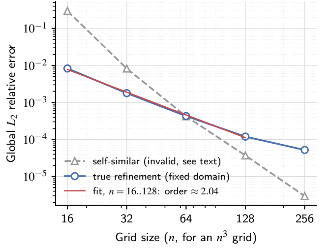
Fig. 1. Global L_2 relative error vs. grid size for the invalid self-similar sweep and the corrected fixed-domain sweep, with the fitted order for the latter.
