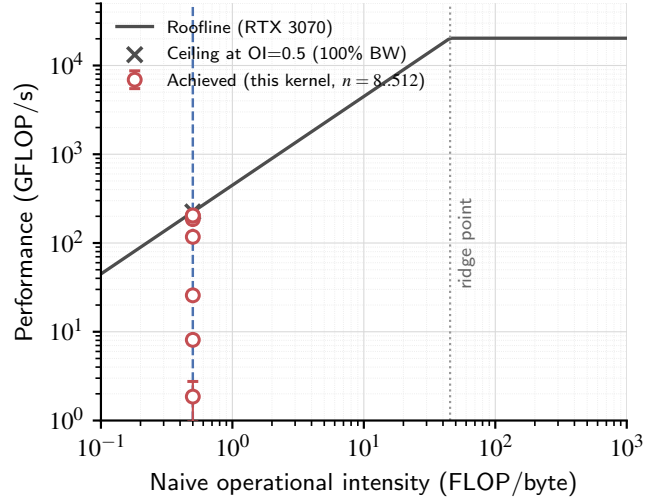
Fig. 4. Roofline model for the RTX 3070. The kernel’s fixed naive operational intensity (dashed line) sits far below the ridge point; achieved performance at each grid size climbs toward the ceiling that intensity imposes as the grid grows.
