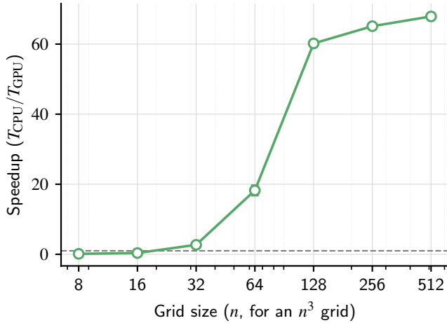
Fig. 3. Speedup (CPU time / GPU time) vs. grid size. The dashed line marks parity.
