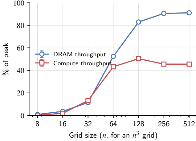
Fig. 5. DRAM and compute throughput (% of peak) vs. grid size. DRAM throughput overtakes and pulls away from compute throughput beyond 64^3 cells.
