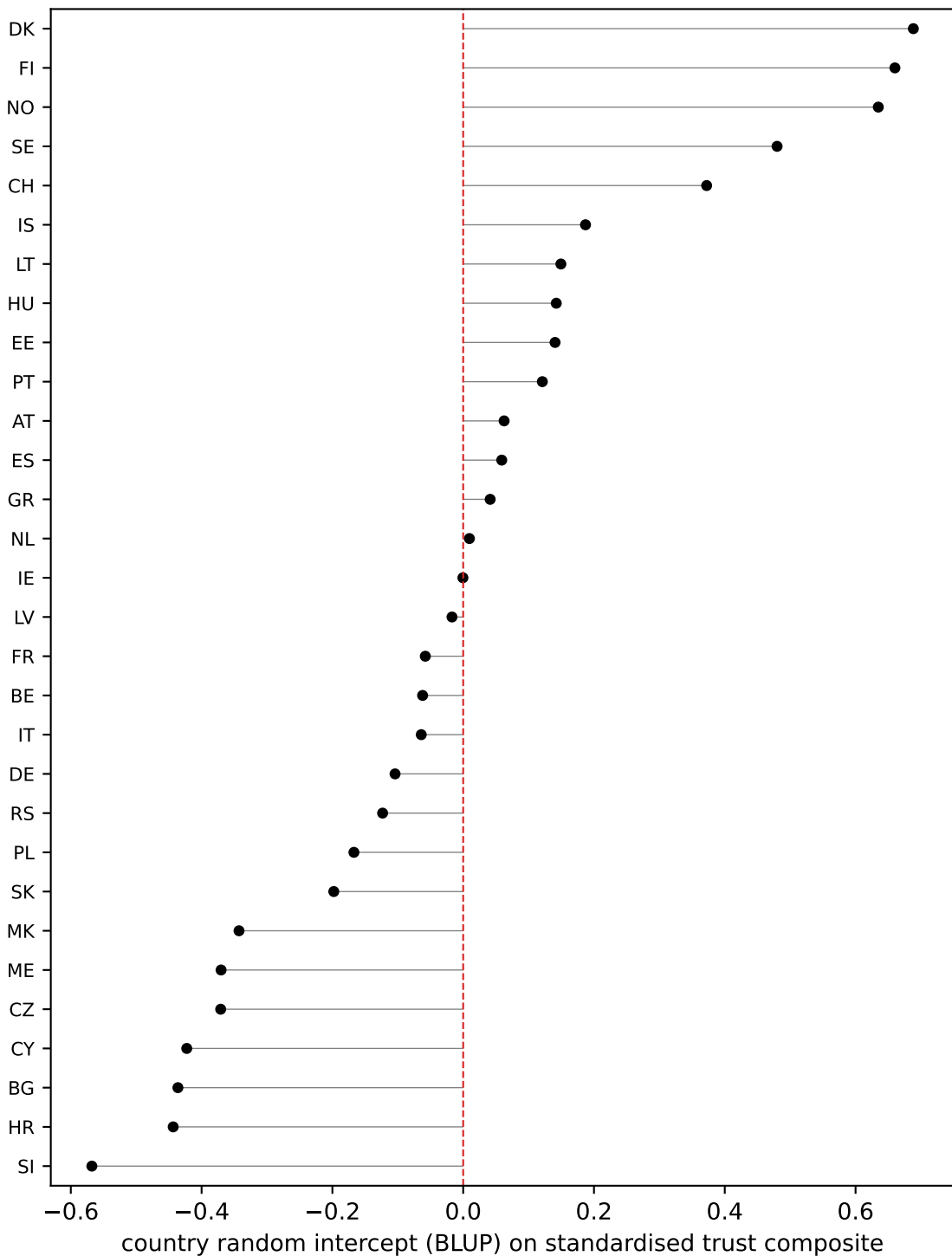
Between-country trust heterogeneity — ranked country BLUPs (M3a)
