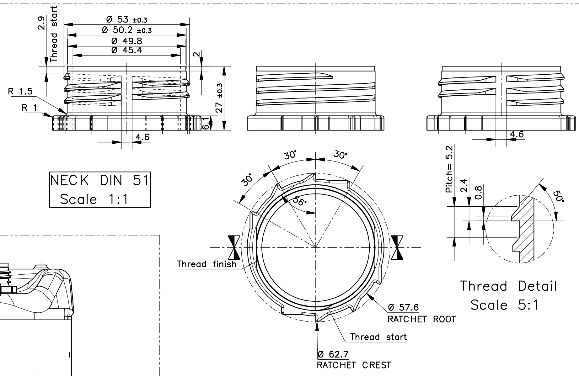
5 LT. VERSION
