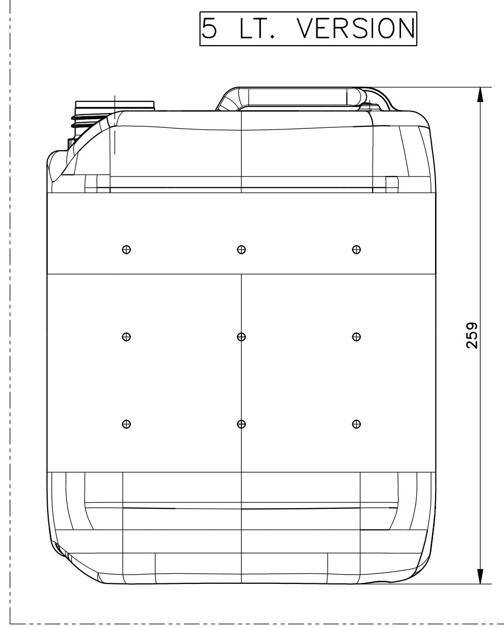
MOULD DIMENSION
