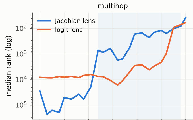
Per-layer median intermediate rank — qwen (shaded: paper workspace band 24–58)
