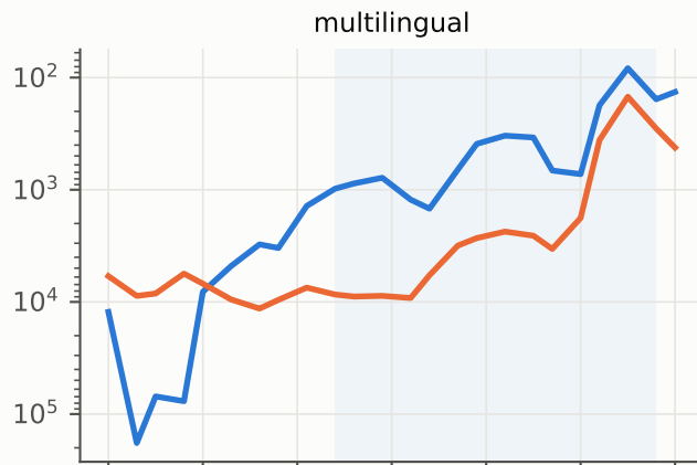
Per-layer median intermediate rank — qwen (shaded: paper workspace band 24–58)
