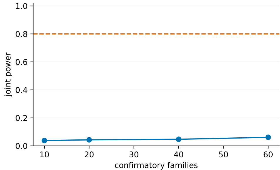
B · Power at candidate SESOI
