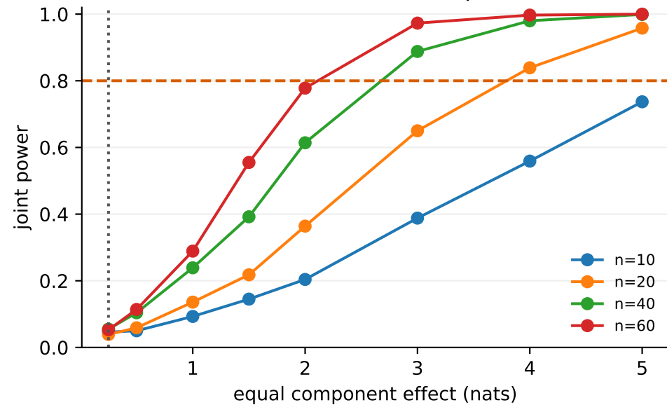
A · Intersection-union power
