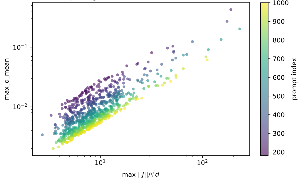
Prompt magnitude versus estimator movement
