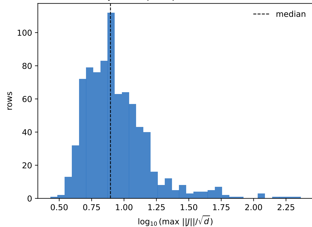
Heavy-tailed prompt-norm distribution
