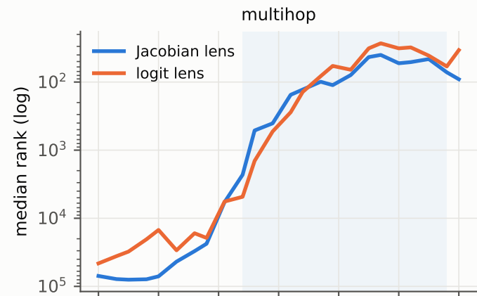
Per-layer median intermediate rank — olmo (shaded: paper workspace band 24-58)
