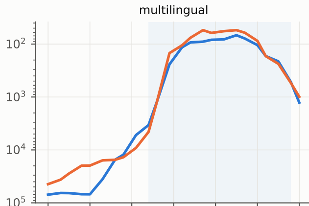
Per-layer median intermediate rank — olmo (shaded: paper workspace band 24-58)
