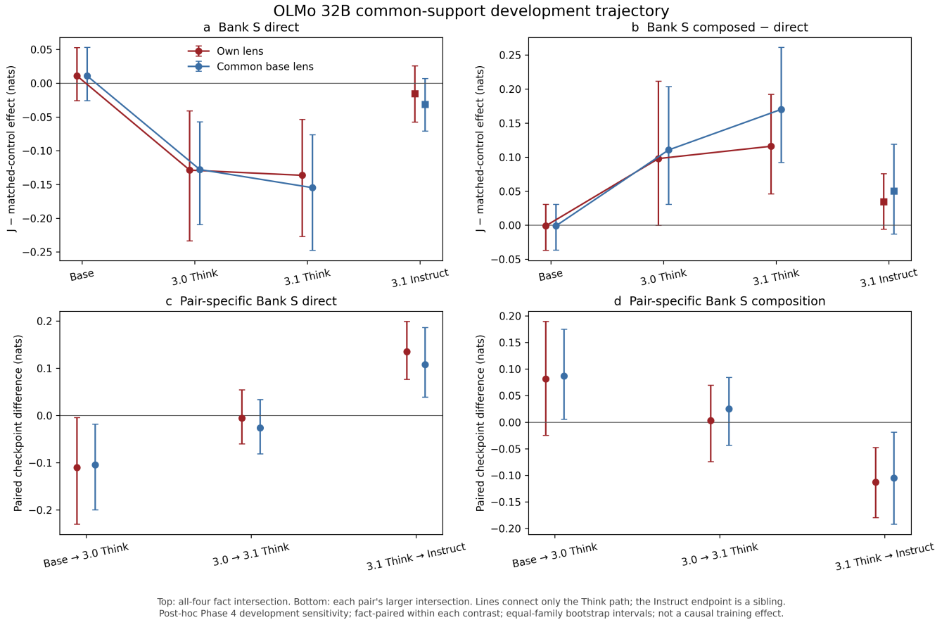
Figure 11: Post-hoc common-support sensitivity. The upper panels use the all-four intersection; the lower panels use larger adjacent-pair intersections. This removes changing fact composition as one explanation, but it does not randomize training.
