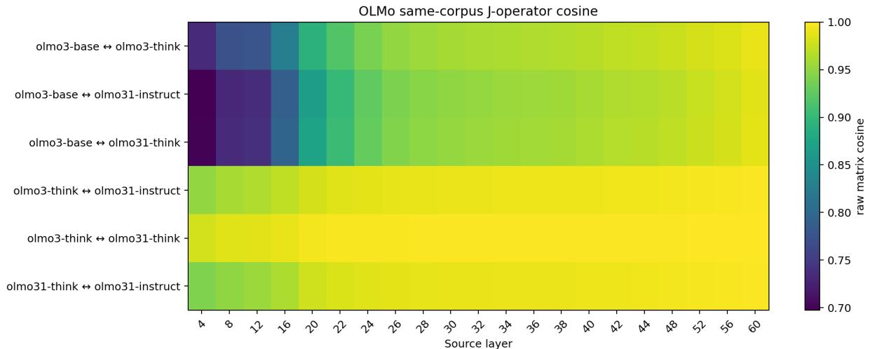
Figure 8: Registered O3 figure 1: raw-operator similarity across checkpoint pairs and layers [ol-geometry-figures-dev-v1]. The transport operators stay broadly similar everywhere (base→3.0 median cosine 0.9614).
