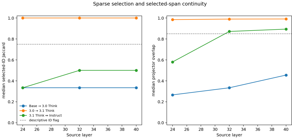
Figure 10: Registered O3 figure 3: what the assay actually selects. Base→3.0 selected-ID Jaccard is 0.3333 at layers 24/32/40 (projector overlap 0.27/0.33/0.45); 3.0→3.1 Jaccard is 1.0 at the same layers [ol-geometry-figures-dev-v1].
