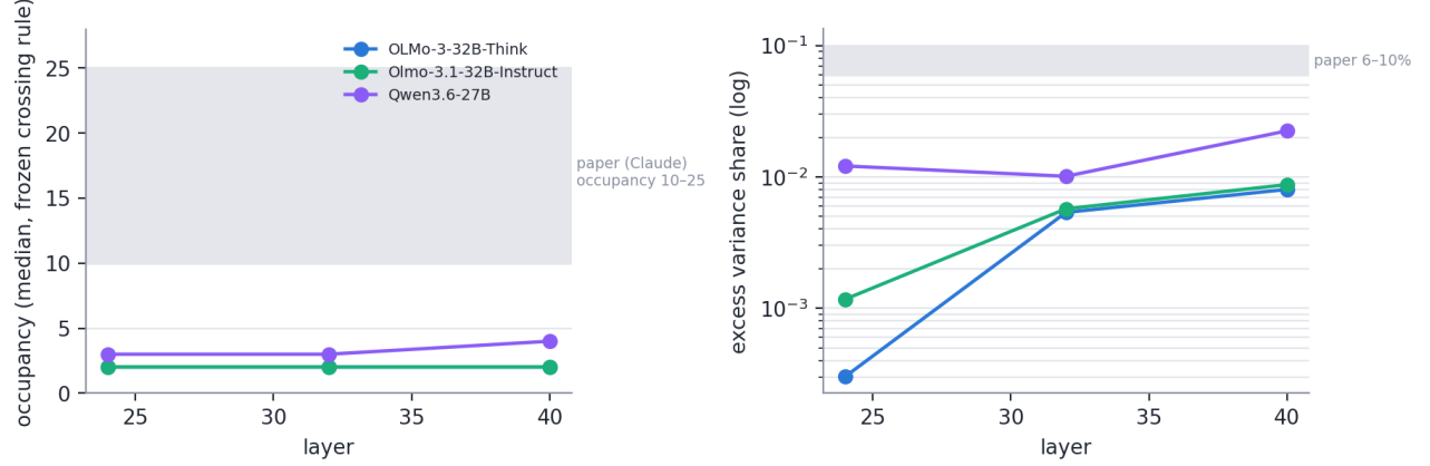
Figure 21: Earlier corrected capacity comparison. OLMo’s occupancy is thin; Qwen sits nearer the lower edge of the source paper’s excess-variance range. Later Phase 4 fit-size work adds a functional-convergence caveat to small-lens comparisons.
