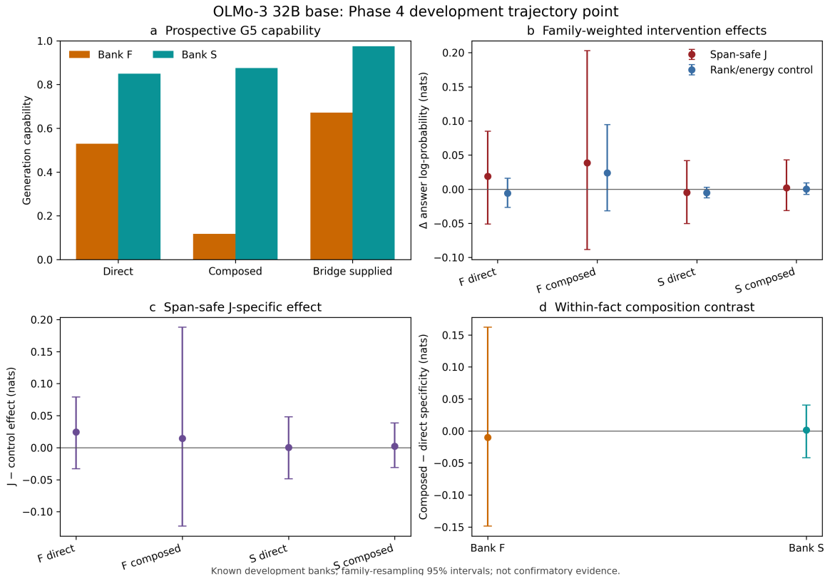
Figure 17: OLMo-3 32B base development point [p4-lineage-analysis-olmo3-base-dev-v1].
