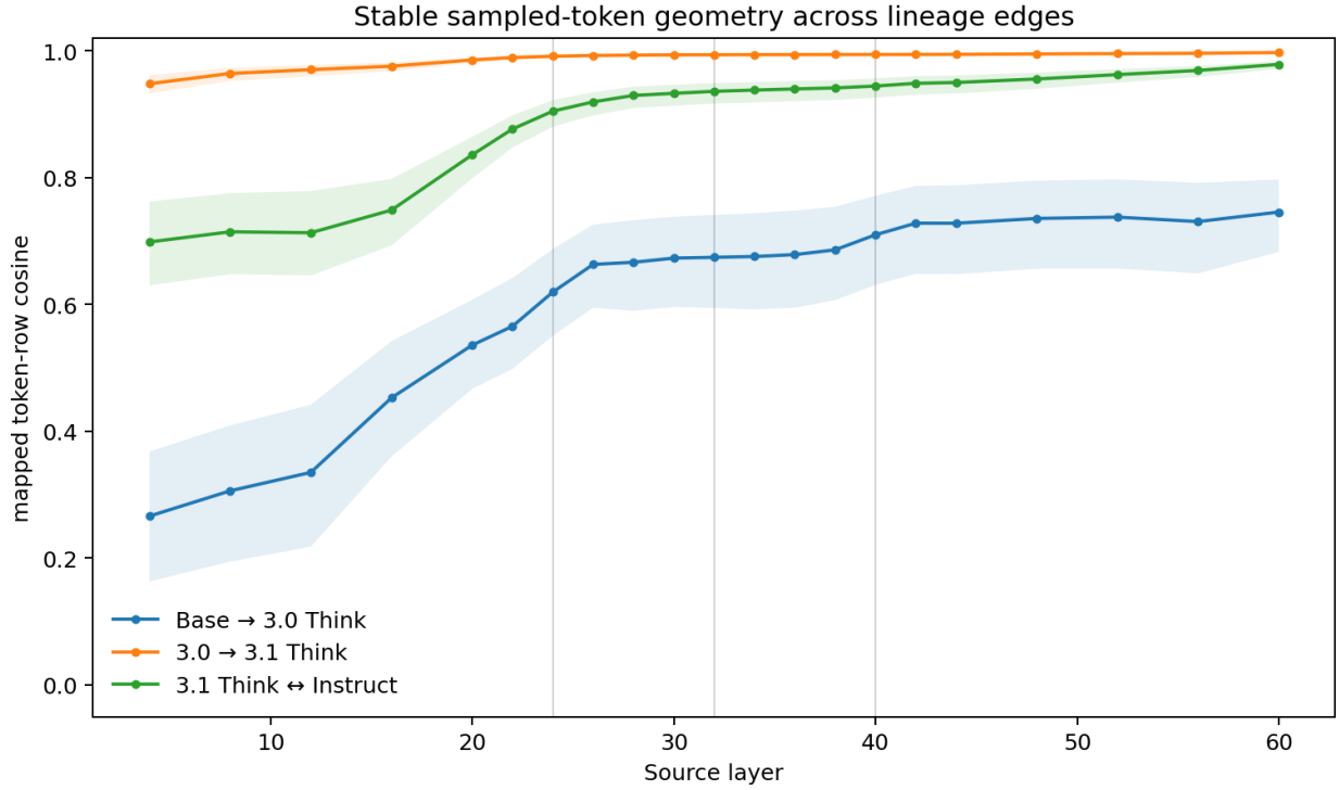
Figure 9: Registered O3 figure 2: J-mapped token-row similarity. Unlike the raw operators, the mapped rows reorganize sharply at base→3.0 (median cosine 0.6744) and then freeze (3.0→3.1 mapped movement 0.006 versus 0.326 for base→3.0) [ol-geometry-figures-dev-v1].
