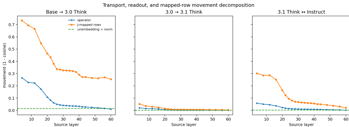
Figure 13: Registered O3 figure 5: readout/transport movement decomposition across the lineage [o1-geometry-figures-dev-v1].
