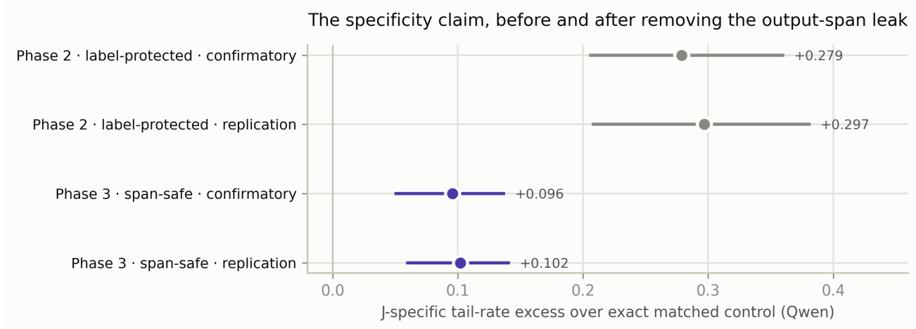
Figure 14: Qwen’s specificity claim before and after output-span repair. The large label-protected Phase 2 tail shrinks under span-safe protection but survives and replicates in Phase 3. This is the confirmatory anchor against which the OLMo lineage development result is interpreted.
