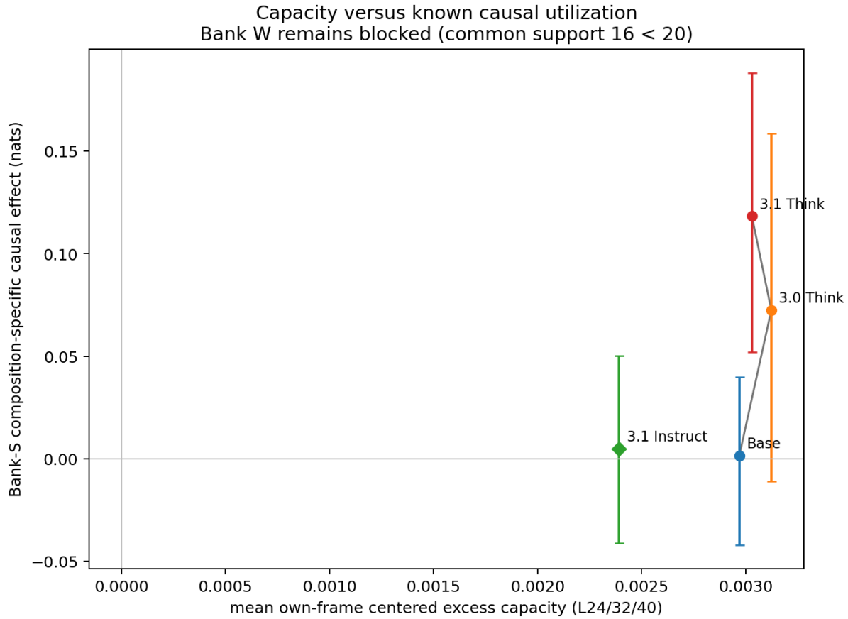
Figure 12: Registered O3 figure 4: measured capacity versus known Bank-S causal dependence, with the 16/20 Bank-W service block annotated [ol-geometry-figures-dev-v1]. The lineage moves almost entirely along the causal axis.
