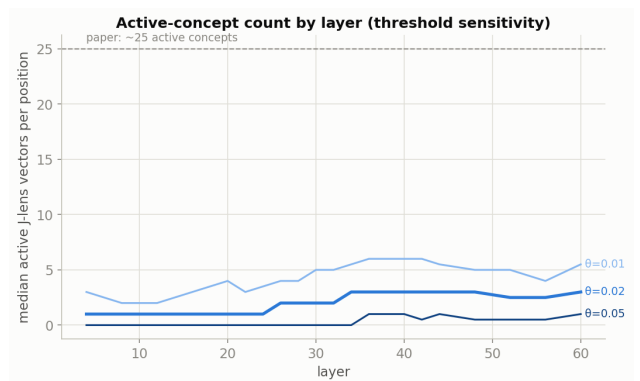
Figure 1: Left: J-space share of activation variance by layer; shaded band = paper’s Claude range (6–10%). Right: median active-concept count by layer under three activation thresholds; dashed line = paper’s \sim 25 .
