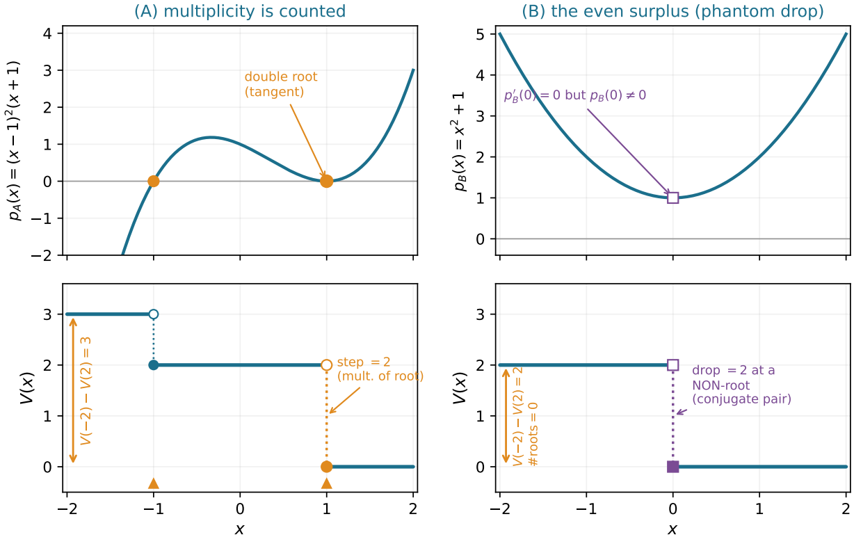
Figure 2: The derivative tower counts roots up to an even surplus. (A) p_A = (x - 1)^2(x + 1) : V drops by 1 at the simple root x = -1 and by 2 at the double root x = 1 (open circle = the value just to the left, filled = the value at the point, on the lower step). The descent over (-2, 2] equals the root count with multiplicity , so the inequality is sharp. (B) p_B = x^2 + 1 , no real root: V still drops by 2, at x = 0 , where the interior member p'_B vanishes but p_B does not—the even surplus, the signature of a conjugate pair. Every plotted sign and count is asserted against exact arithmetic before drawing.
