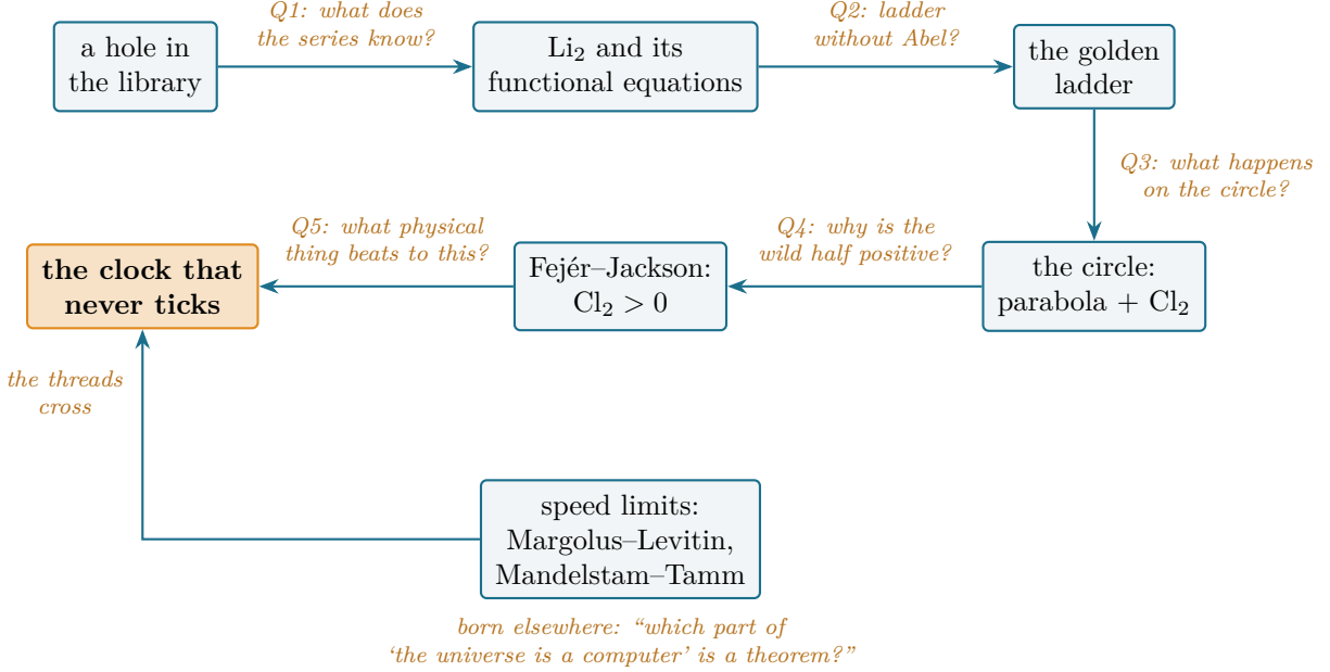
Figure 1: The honest map. The dilogarithm thread runs along the top and back; the quantum thread (bottom) was born independently and crossed it at the end — the crossing, not the chain, is where the title theorem lives. Every node is a block of sorry-free Lean .
