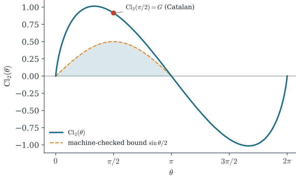
Figure 2: The Clausen function on [0, 2\pi] with the machine-checked lower bound \sin(\theta)/2 (shaded) on (0, \pi) , and Catalan’s constant at the quarter circle. The generating script asserts the bound on a 400-point grid at 30 digits.
