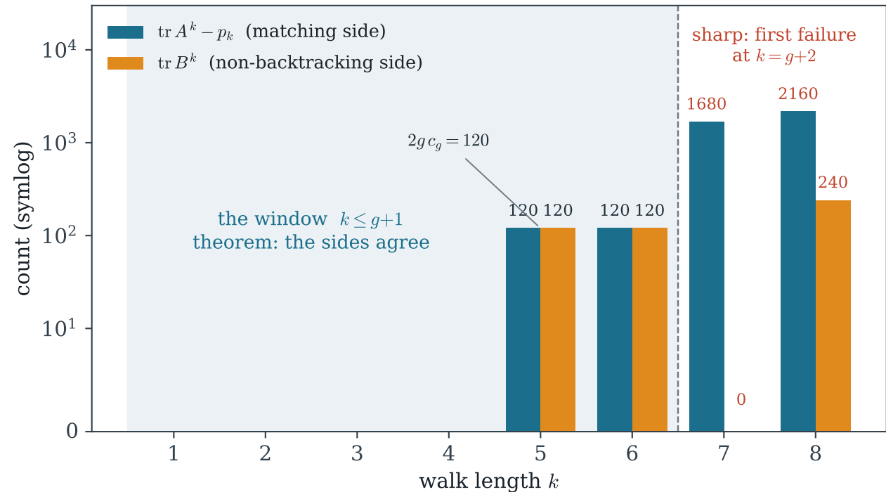
Petersen graph ( g = 5 ): the gap law on its sharp window
