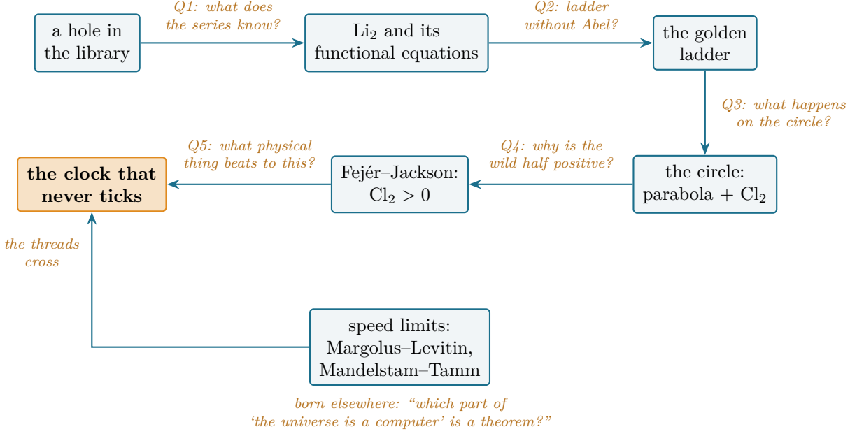
Figure 1: The honest map. The dilogarithm thread runs along the top and back; the quantum thread (bottom) was born independently and crossed it at the end — the crossing, not the chain, is where the title theorem lives. Every node is a block of sorry-free Lean .
