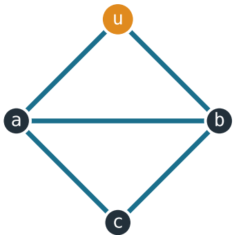
G = \text{diamond} , root u
