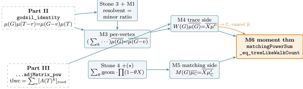
Figure 1: Formal-dependency roadmap. Two external inputs (Parts II and III, dashed) feed a trace column and a matching column; each terminates at the same reflected derivative \overline{X\mu'} (M4 over \mathbb{R} , M5 over \mathbb{C} ); the base change \mathbb{R} \rightarrow \mathbb{C} and cancellation of the unit \overline{\mu} close the moment theorem (M6, amber). Every box is a sorry -free Lean result; cf. Table 2.
