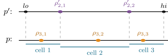
Figure 2: The recursion, for \deg p = 3 . The two virtual roots of p' (plum) together with the fences lo, hi cut [lo, hi] into three cells; on each cell p' keeps a constant sign, so \mathcal{R}_d returns one virtual root of p (amber). Each \rho_{3,j} lies in its own cell—this is what makes them come out sorted and interlaced with the \rho'_{2,j} .
