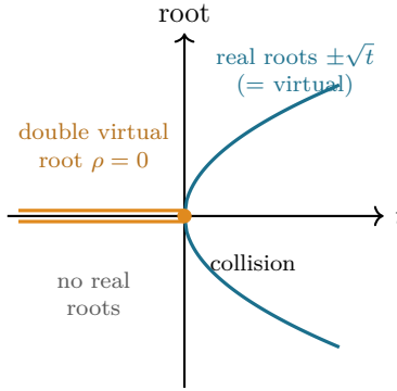
Figure 4: Roots that are always there, as a parameter moves. For p_t = x^2 - t the two real roots \pm\sqrt{t} (teal) exist only for t \geq 0 and vanish as t drops below 0; the two virtual roots (amber) persist for all t , coinciding with the real roots when t \geq 0 and colliding into the double virtual root \rho = 0 for t < 0 . The real-root count jumps 2 \rightarrow 0 at t = 0 ; the virtual-root count stays 2. The collision at t = 0 is exactly where a conjugate pair forms—the source of the even Budan–Fourier surplus. (A different view of the same phenomenon as Figure 1, now in motion.)
