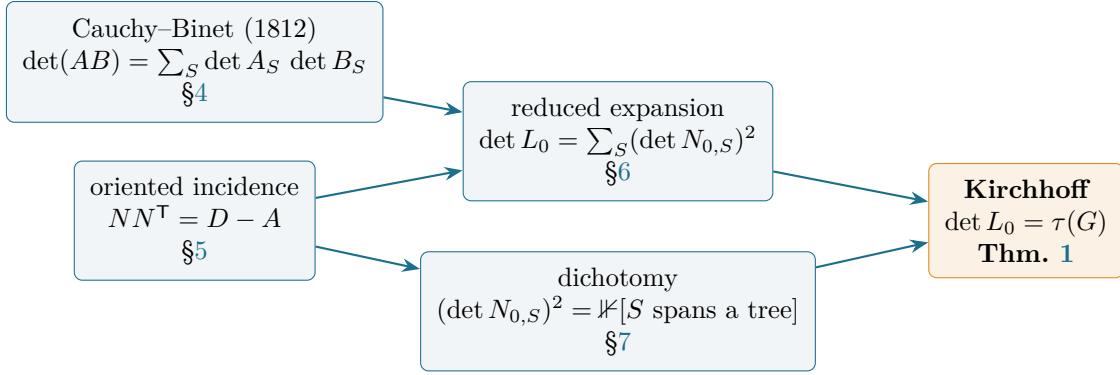
Figure 2: The proof chain. Two classical ingredients combine into the sum-of-squares expansion; the dichotomy decides each summand; the count falls out.
