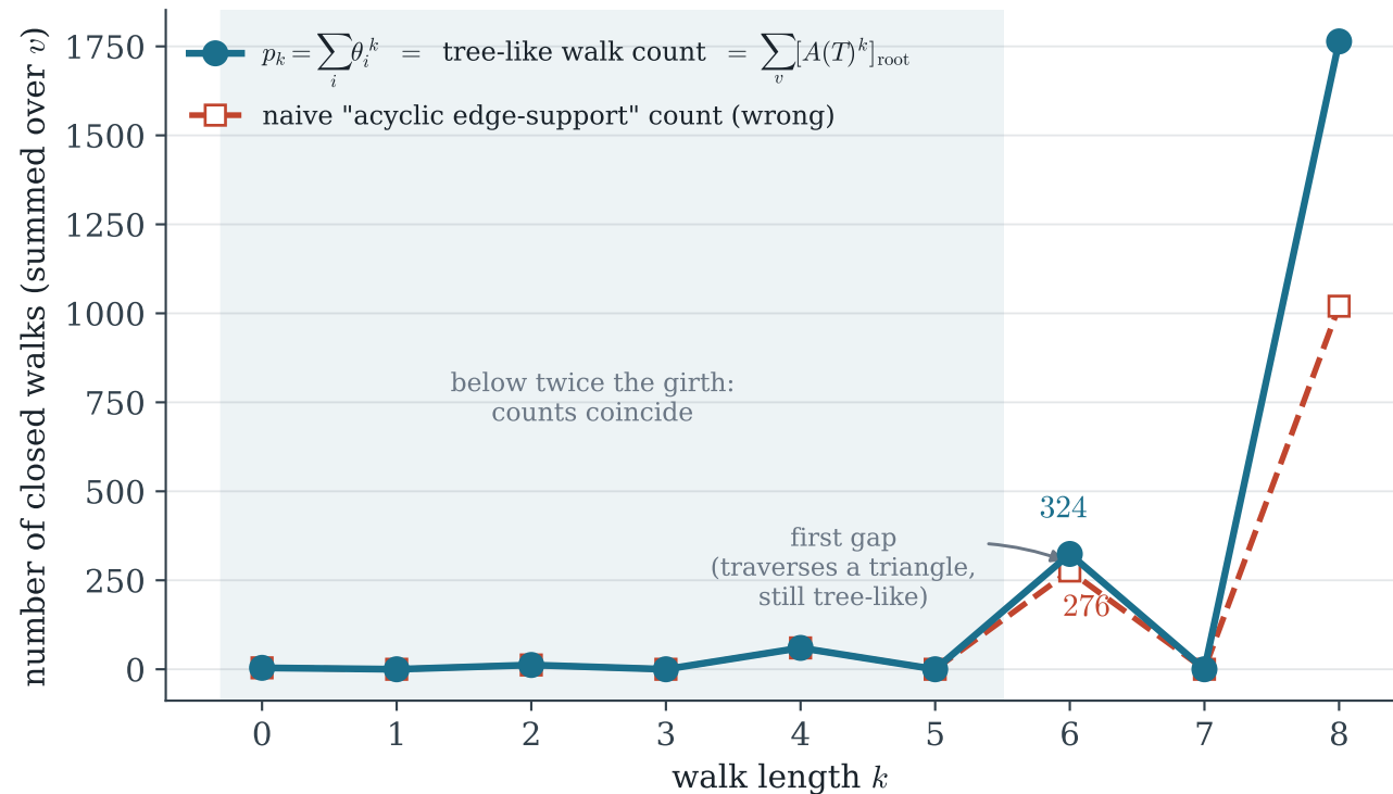
K_4 : the corrected count vs. the plausible-but-wrong one
