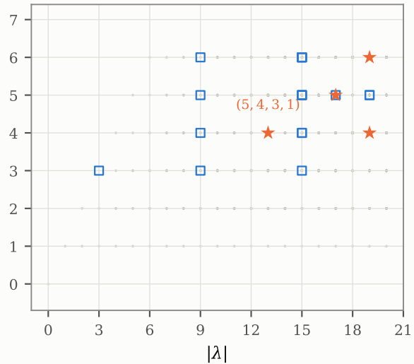
r = 2, N = 6 : 4 of 1513 shapes
