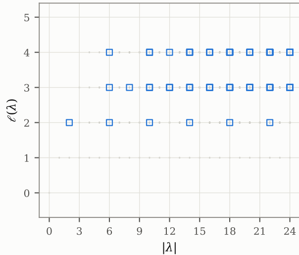
r = 1, N = 4 : no such shape in 1292
