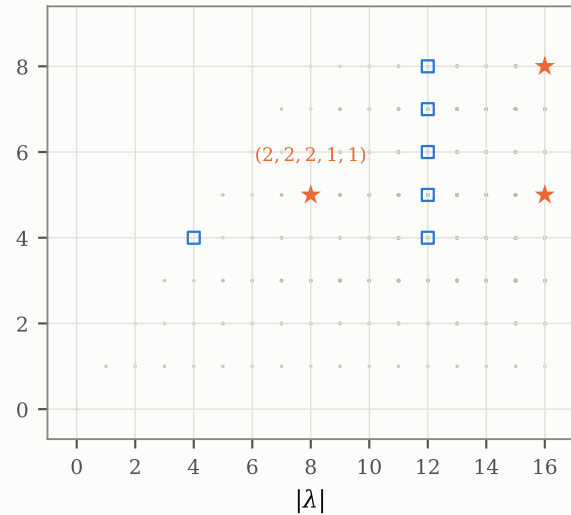
r = 3, N = 8 : 3 of 795 shapes
