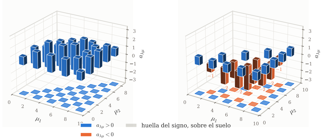
(a) \lambda = (9, 8, 8, 6, 0, 0) : un carácter genuino, todos los a_{\lambda\mu} > 0 (b) \lambda = (9, 9, 8, 6, 0, 0) : propiamente virtual
