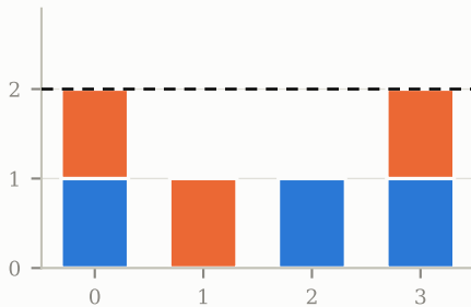
A_9(40), p=2: d=2, e=4 not Gorenstein
