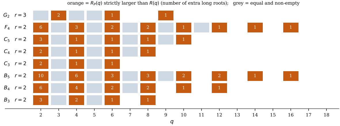
Figure 6: B , C and F_4 part company only at even q ; G_2 only at q = 3, 6, 9 , the multiples of its r = 3 . The number in each orange cell is how many extra long roots R_P(q) carries.
