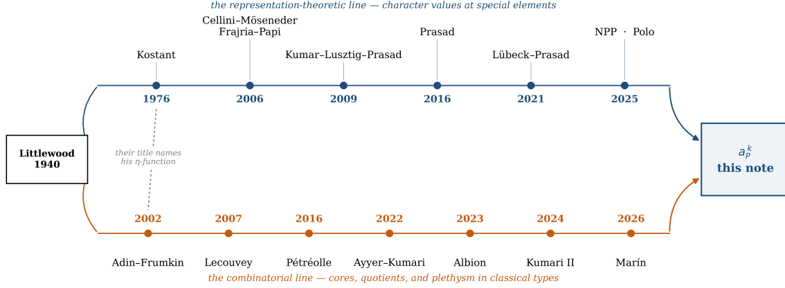
Figure 1: The two lines. The axis is time and each node carries a name and its year of publication , the dates being those of the bibliography below. Above, character values at special elements: Kostant [12] fixes a_Q and a_P and proves the values are \{0, \pm 1\} ; Cellini–Möseneder Frajria–Papi [6] evaluate the character at a_P outright; Kumar–Lusztig–Prasad [13] make twisted and folded the same word; Prasad [21, 22] supplies the geometry of \rho and the residue criterion on \mathrm{GL}_n ; Lübeck–Prasad [15] carry it to S_{2n} and B_n ; and NPP [18] and Polo [20] arrive in 2025. Below, the combinatorial side: cores in type A [1]; the \ell -quotient in classical types through plethysm [9, 10]; the Macdonald identity of type \tilde{C} [19]; and characters twisted by roots of unity [3, 2, 8]. Littlewood 1940 sits outside both because it feeds both, and the box on the right is this note: the two arrows into it are the two things it needs, the element from above and the alphabet from below. The node to read first is 2006. Corollary 3.2 of [6] is already the vanishing criterion and the sign, in every type, and on the root statistic — this line, not the coroot line. Everything this note has to add begins one step further along: at the powers a_P^k , where \rho stops being regular. In the coroot statistic the criterion is Corollary 3.7 of [18], for every integer. The dotted edge is the crossing of 2002: Adin–Frumkin’s title is Rim hook tableaux and Kostant’s \eta -function coefficients , a combinatorial paper taking its coefficients from the 1976 paper where both of Kostant’s elements are defined. The two lines do see each other, and it is worth being exact about how much: [18] cites Ayyer–Kumari; Kumari’s papers are motivated by a conjecture of Wagh and Prasad; and Ayyer–Kumari [3] open by saying that Littlewood and Prasad considered their factorisations “ motivated by a celebrated result of Kostant ”. So the connection Prasad–Kostant is on the record on both sides. What is not on either side is the identification of §4: a_P^k as d \cdot \mu_q less two letters, read on the line of \rho . [figs.py]
