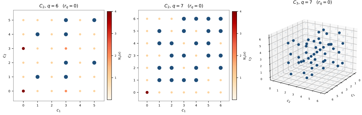
Figure 5: The criterion is a point avoiding walls. Each dot is one weight modulo q , in the coordinates x = \sum_j c_j \omega_j ; blue means the character does not vanish there. The colour of the others is N_q(x) , the number of walls the point does lie on — the darker the point, the more divisibilities \lambda forces beyond what \rho already forced. Left, C_2 at q = 6 , which is a_P itself: 8 survivors where \prod_i (q - m_i) would give 15. Middle, C_2 at q = 7 : 24 , and the product gives 24. Right, the same picture one dimension up, C_3 at q = 7 : 48 , and the product gives 48. The parity of q , and nothing else, separates the two regimes. [fig_walls.py]
