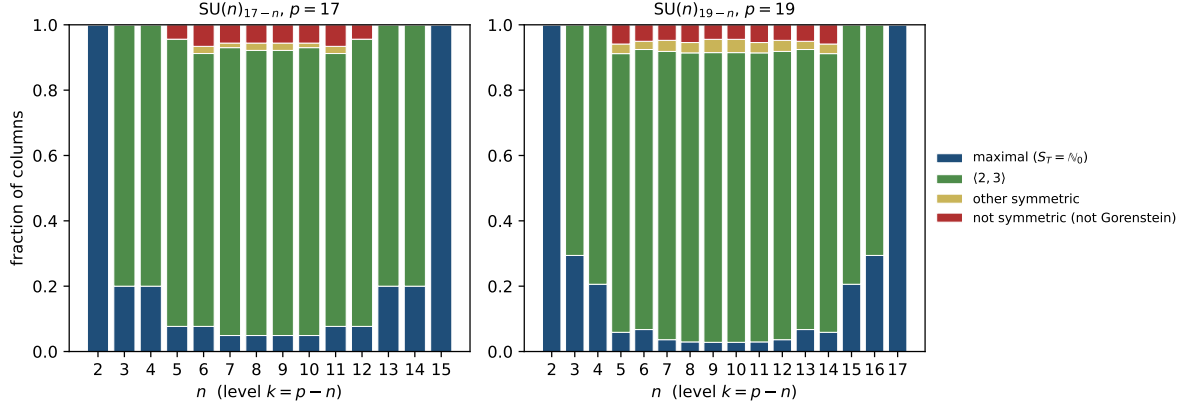
Figure 2: The columns of SU(n)_{p-n} by the semigroup S_T of their spectrum, computed with the exact formula of Theorem 3; each centred spectrum stands for n columns. Maximal columns (blue) have A_\mu = \mathcal{O}_\mu ; \langle 2, 3 \rangle (green) has one gap; the other symmetric semigroups (gold) are Gorenstein with more gaps; the red ones are not Gorenstein. The bars for n and p - n agree, as level–rank duality demands.
