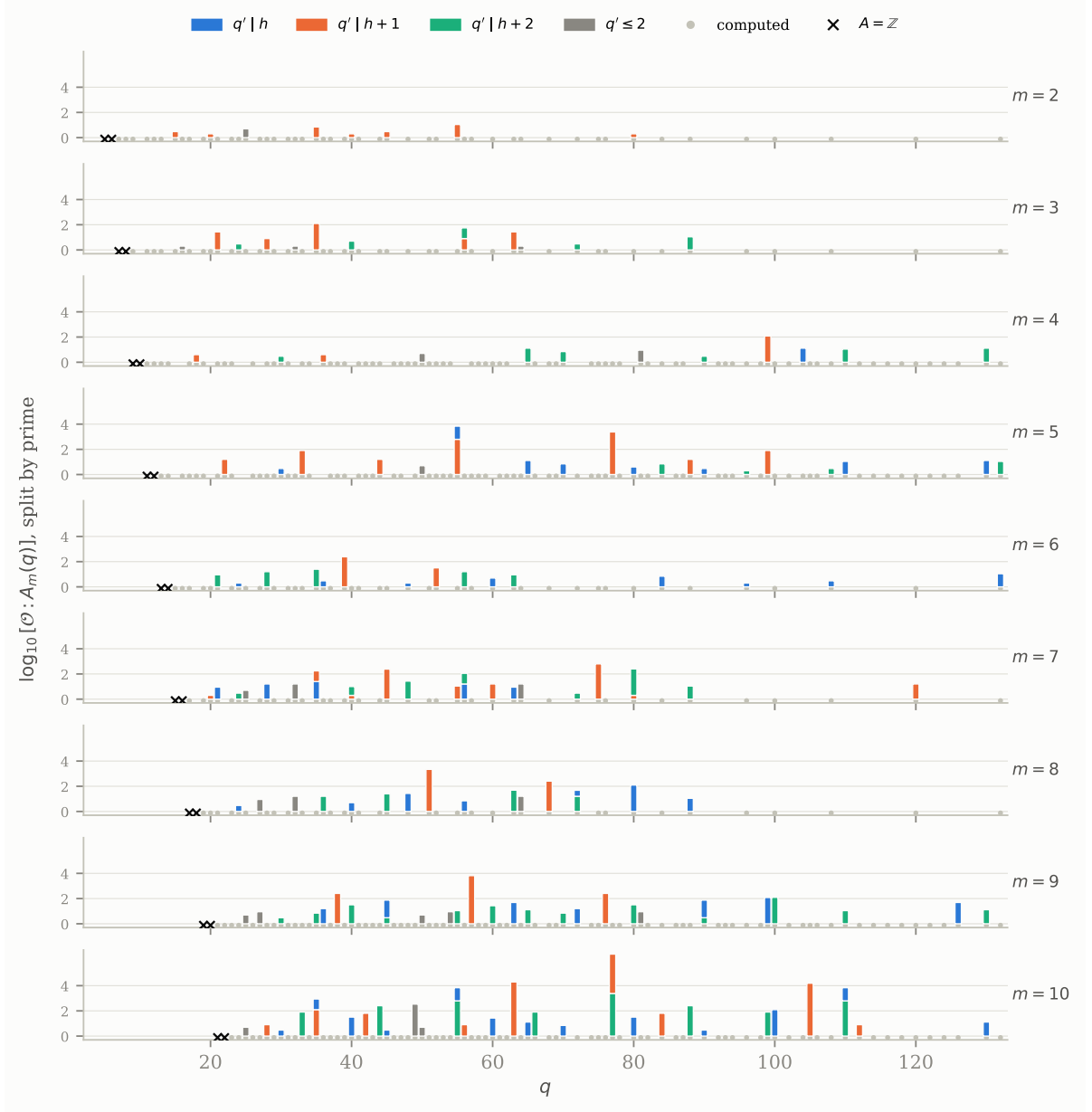
Figure 3: The index [\mathcal{O} : A_m(q)] for 2 \leq m \leq 10 and q \leq 132 (558 orders with a lattice computation, 156 of them with index > 1 ; the equality with the 156 half-period cases of §6.2 is a coincidence), one panel per m . Each bar is stacked by the primes p of the index, each segment of height v_p \cdot \log_{10} p and coloured by the family of q' = q/p^v ; grey segments are primes with q' \leq 2 , outside the theorems. Dots mark computed q (no bar: index 1); crosses mark A = \mathbb{Z} . Every coloured segment lies over a pair with q' \mid h, h+1, h+2 .
