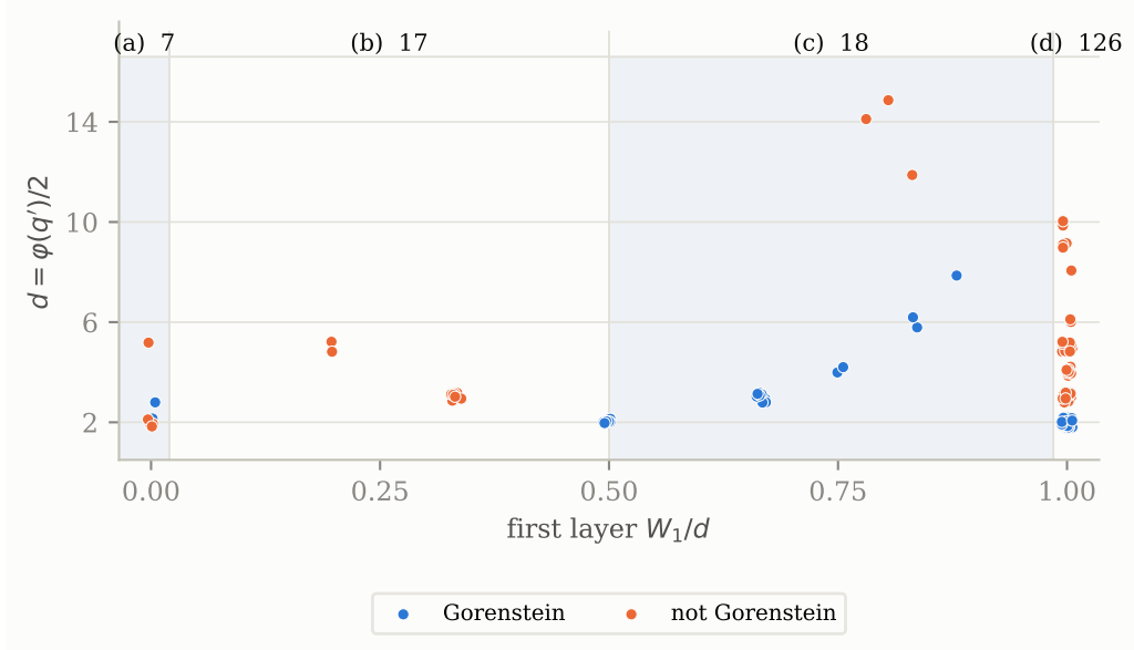
Figure 8: Where the first layer falls, on the 168 measured profiles with q' \notin \{1, 2, 3, 4, 6\} , and what decides the exponent in each band: (a) W_1 = 0 , the zone of the ladder and the descent (Propositions 19 and 20); (b) 0 < W_1 \leq d/2 , where Corollary 18 needs its second clause W_2 = d ; (c) d/2 < W_1 < d , where Proposition 8(b) gives e = 2 ; (d) W_1 = d , where e = 1 . Colour marks whether the local ring is Gorenstein. The vertical axis is d = \varphi(q')/2 , with a small jitter so that repeated pairs separate.
