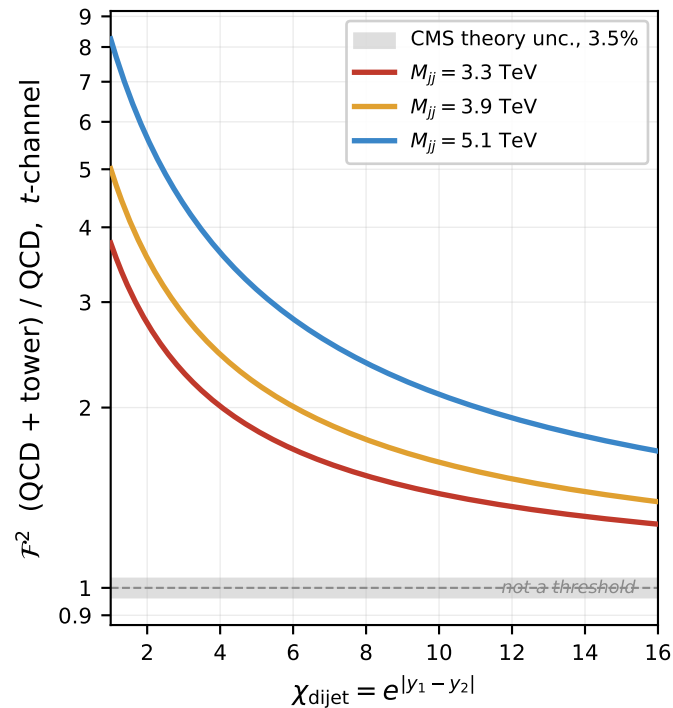
escape branch, 1/R_5 = 3.97 TeV
