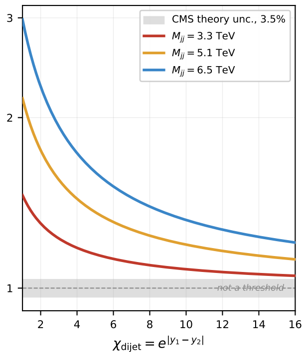
ceiling at the measured mass, 1/R_5 = 9.09 TeV
