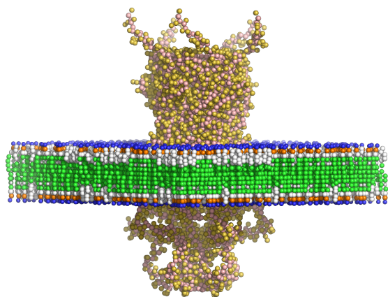
(a) Side view: Extracellular (top), lipid bilayer (middle) and intracellular (bottom) regions.
