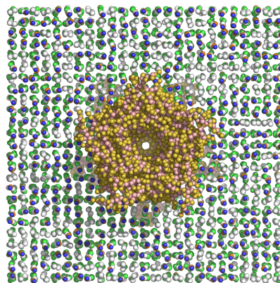
(b) Top view: The tapering of protein's structure.
