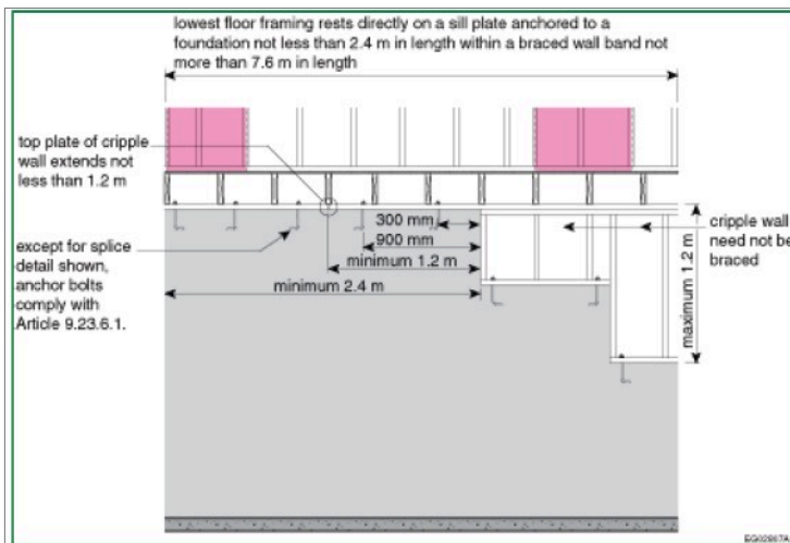
Figure A-9.23.13.9.(1)
