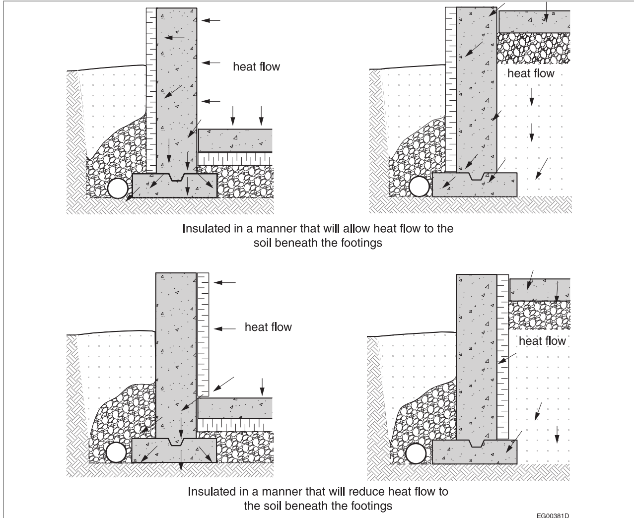
Figure A-9.12.2.2.(2)
