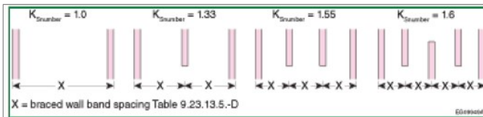
Figure A-9.23.13.7(4)-B Adjustment for Number of Braced Wall Bands Resisting Seismic Load
