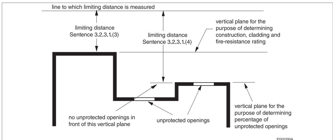
Figure A-3.2.3.1.(4) Spatial separation design
