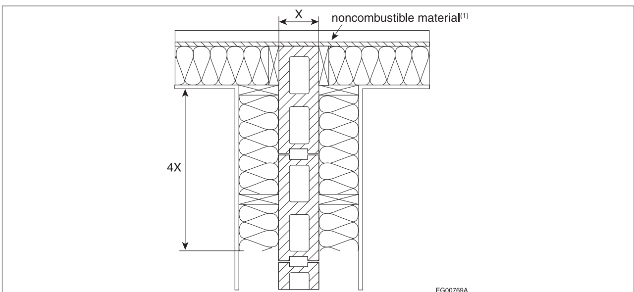
Figure A-9.36.2.5.(2)-A Penetrating element insulated on both sides
