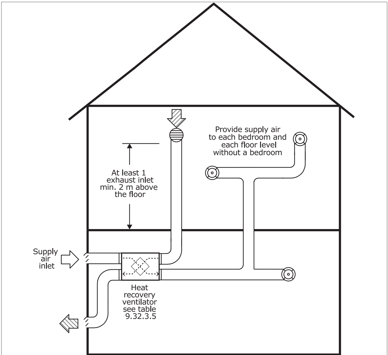
Figure 9.32.3.4.(4) Heat Recovery Ventilator Supply Air Distribution
