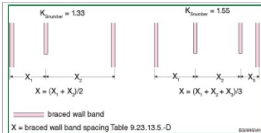
Figure A-9.23.13.7(4)-C Calculation of Mean Braced Wall Band Spacing for Seismic When the Spacings between Adjacent Braced Wall Bands are Not Uniform
