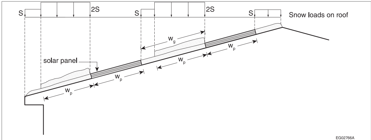
Figure A-4.1.6.16.(4)(b) Snow loads for a sloped roof with Parallel Flush solar panels where w_g \geq w_p
