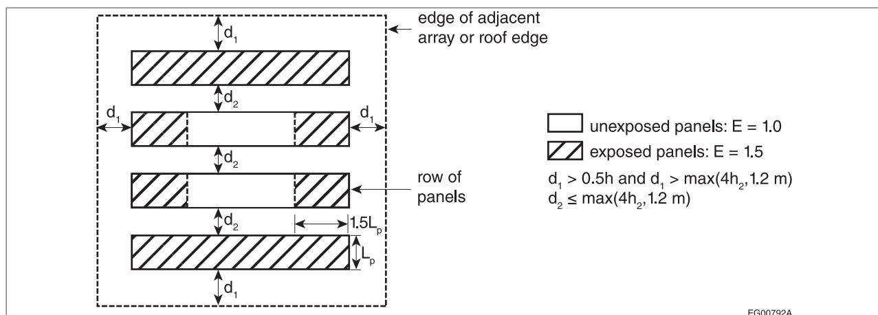
Figure A-4.1.7.13. Plan view of a roof-mounted solar array with exposed and unexposed panels
