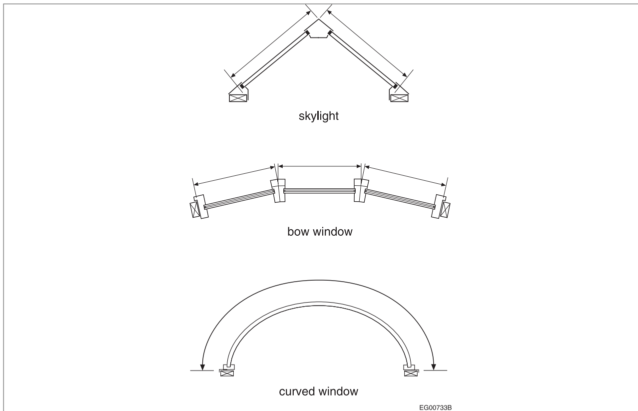
Figure A-9.36.2.3.(5)
