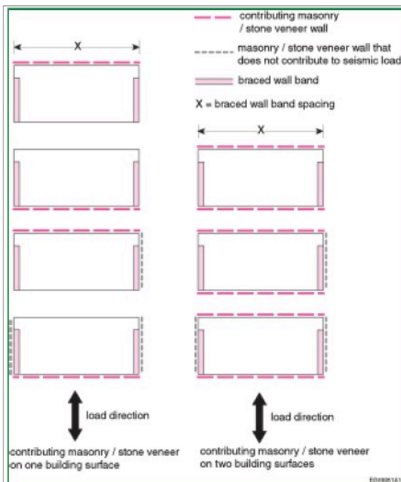
Figure A-9.23.13.7(4)-D Masonry Veneer or Stone Veneer Walls that Contribute to Seismic Force Applied on a Building
