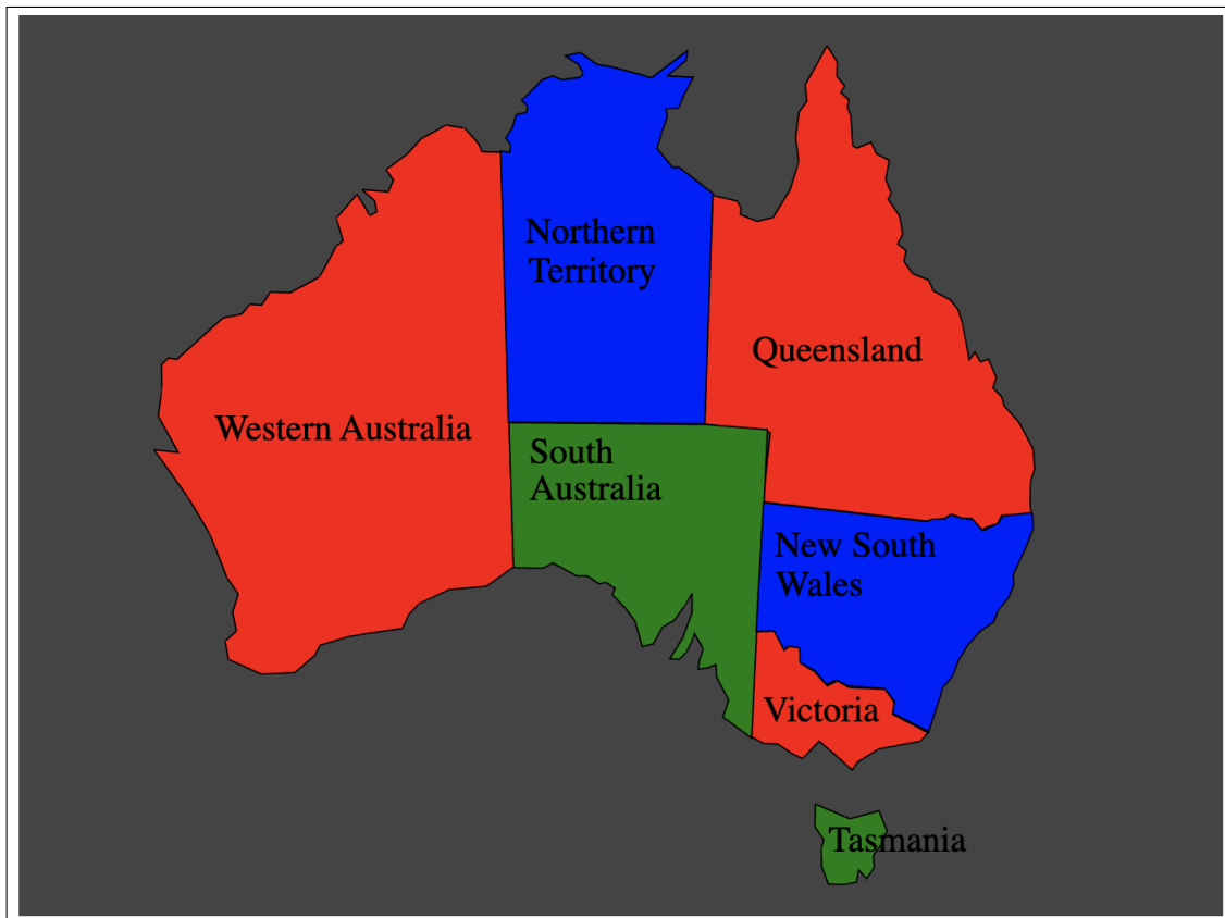
Figure 5.14: A map coloring for Australia.
