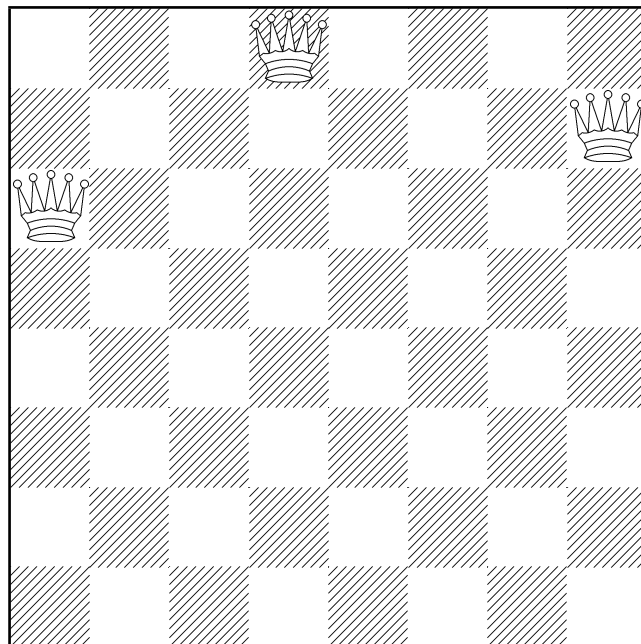
Figure 5.16: The partial assignment \{Q_1 \mapsto 4, Q_2 \mapsto 8, Q_3 \mapsto 1\} .
