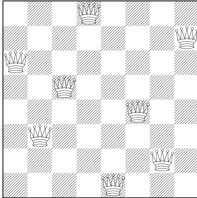
Figure 5.15: A solution of the eight queens problem.
