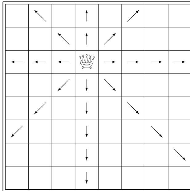
Figure 4.19: The 8-Queens-Problem.
