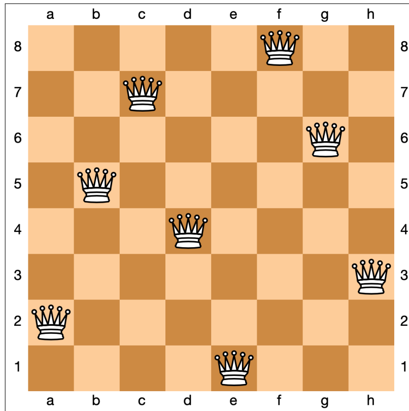
Figure 4.31: A solution of the 8-queens-problem.
