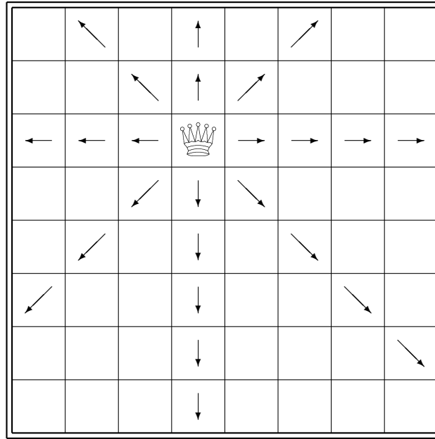
Figure 4.21: The 8-Queens-Problem.
