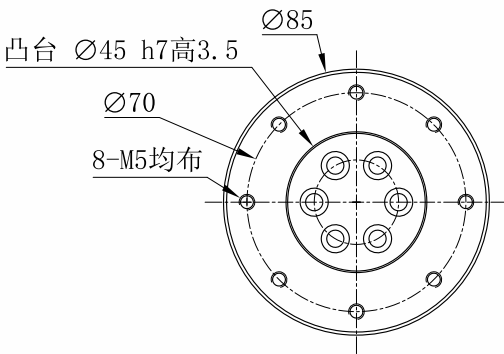
Flange Dimensions
