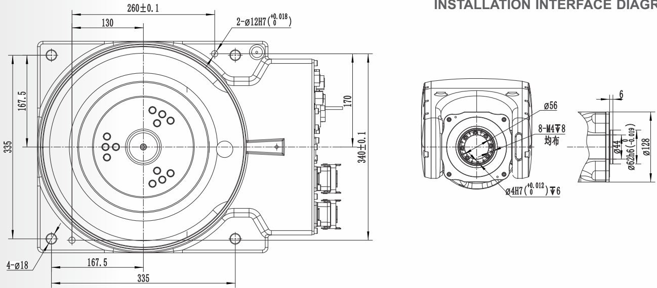
Installation Dimension of Base
