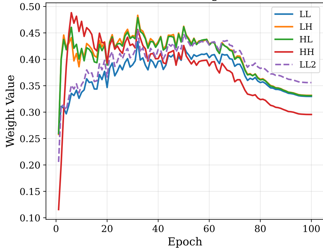
Wavelet Subband Weight Evolution
