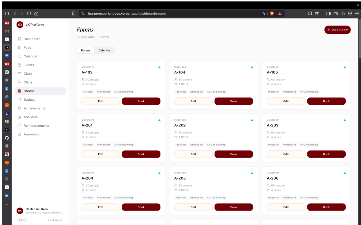
Rooms list -- 57 rooms with capacity cards, amenity tags, and green availability indicator
