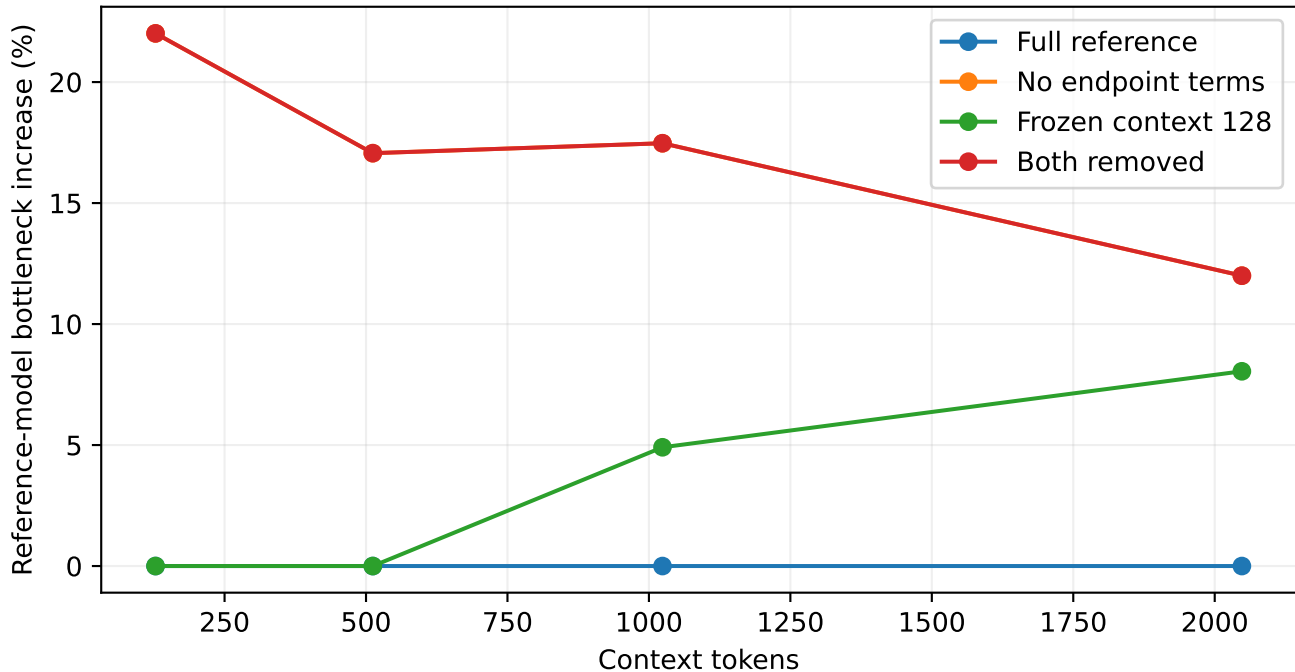
Separated cost-model ablations — analytical, not runtime gains
