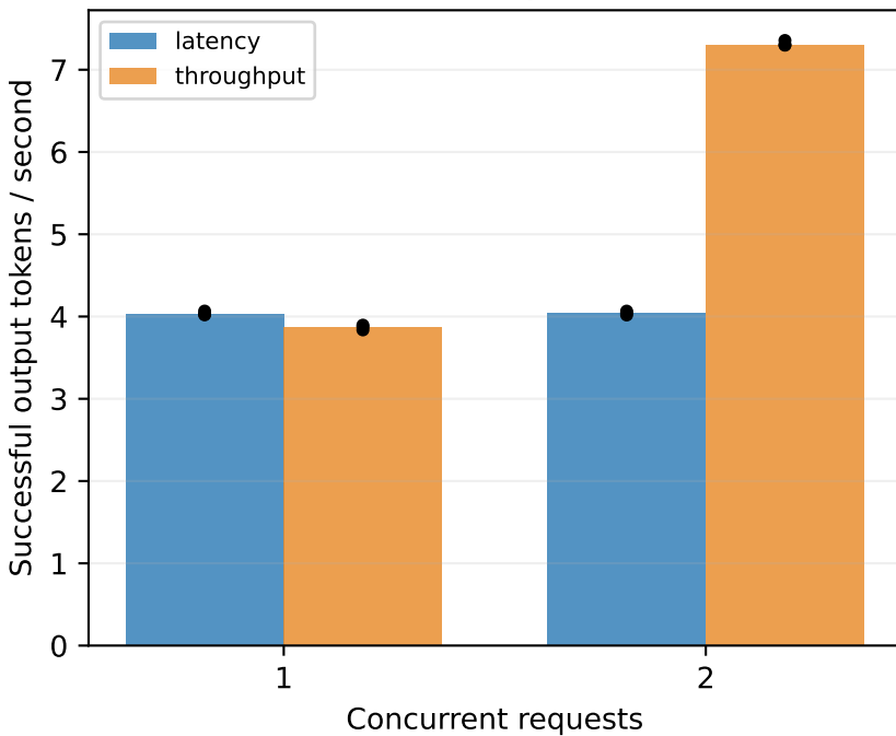
Stable: 32 output tokens
