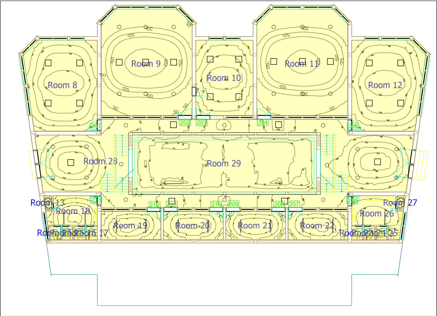
Storey 2 , Illuminance values in [lx]
