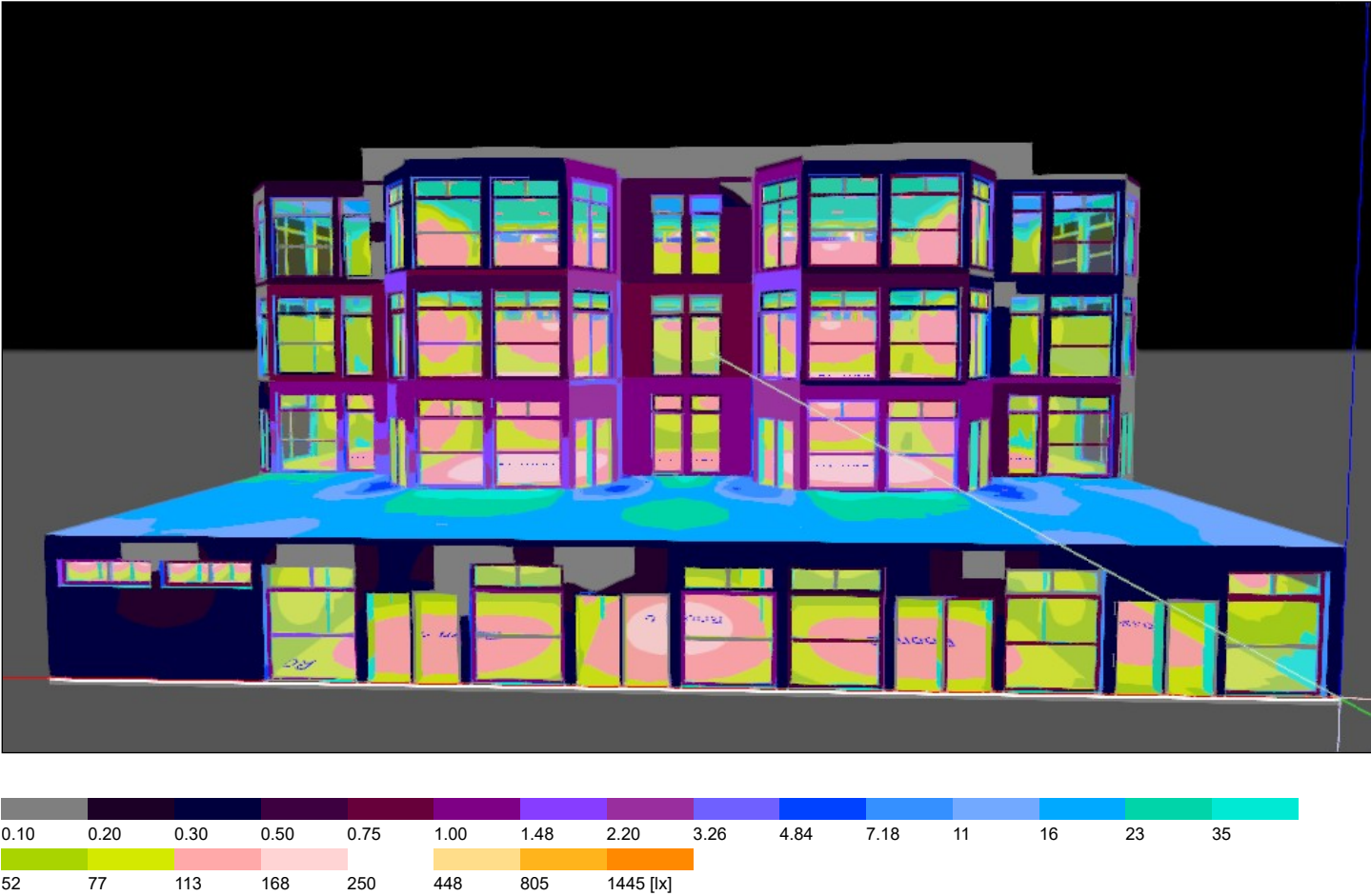
Building 1, Illuminance values in [lx]
