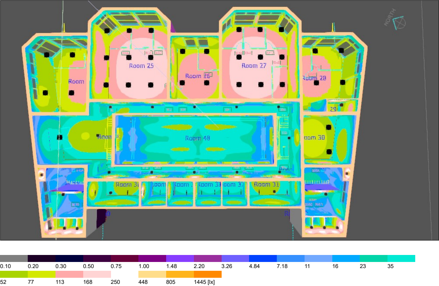
Storey 3(3D), Illuminance values in [lx]
