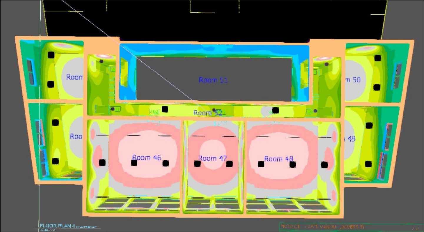
Storey 4 (3D), Illuminance values in [lx]
