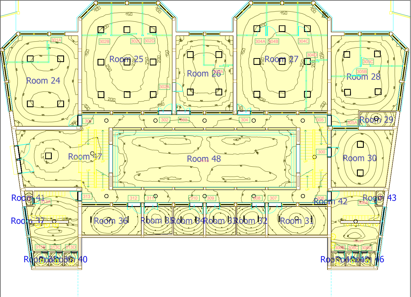
Storey 3, Illuminance values in [lx]
