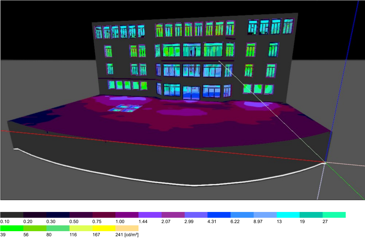
Building 2, Luminance values in [cd/m²]
