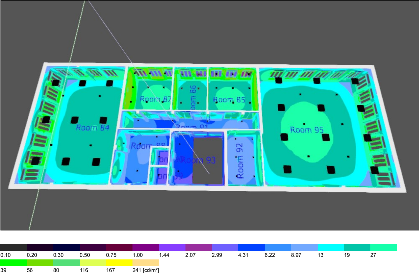
3rd floor (3D), Luminance values in [cd/m²]
