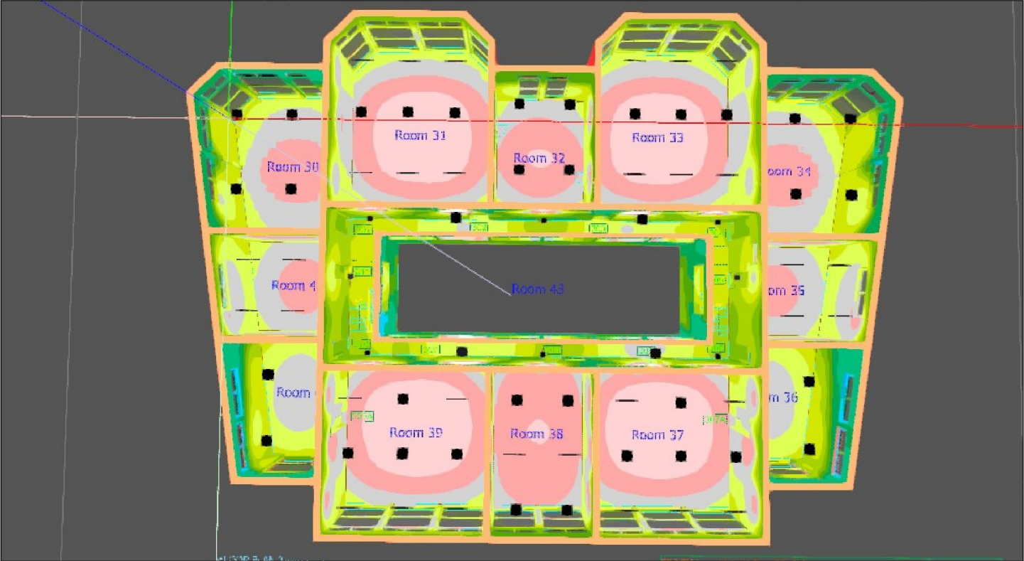
Storey 3 (3D), Illuminance values in [lx]
