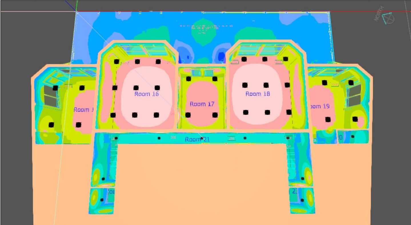
Storey 2 (3D), Illuminance values in [lx]
