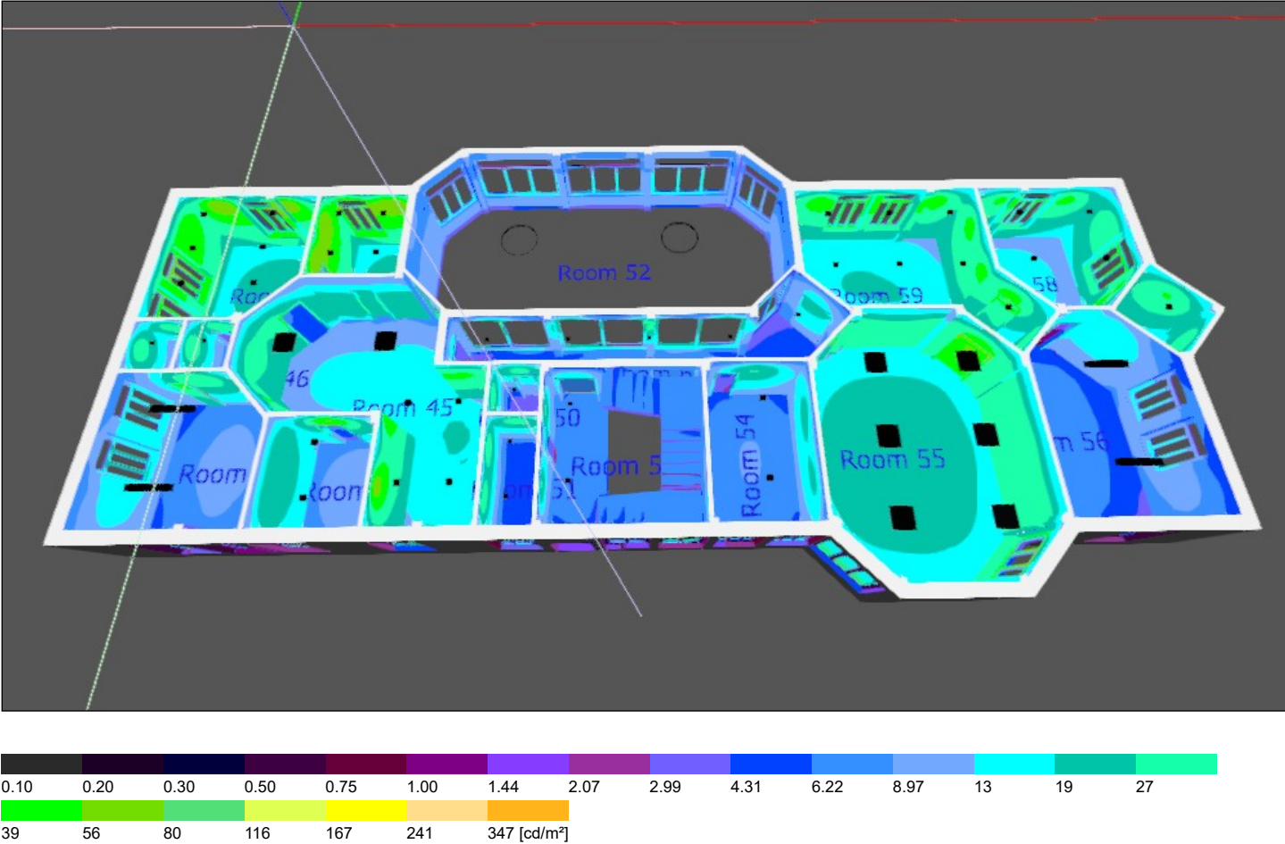
1st floor (3D), Luminance values in [cd/m²]
