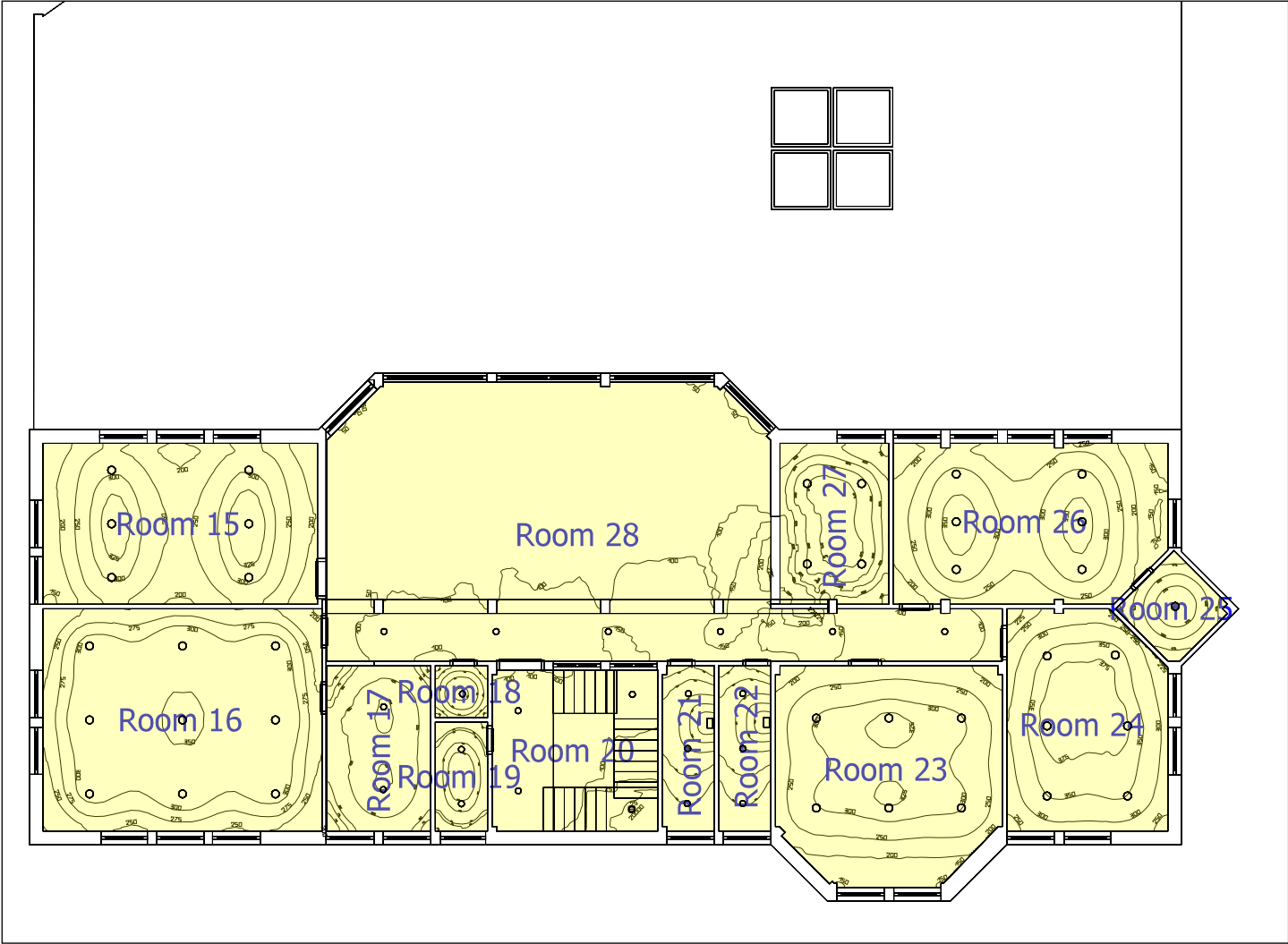
ground floor, Luminance values in [cd/m²]
