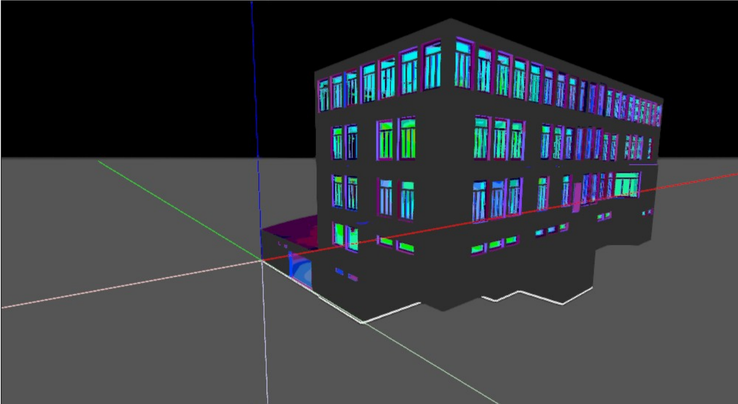
Building 2 (opp), Luminance values in [cd/m²]
