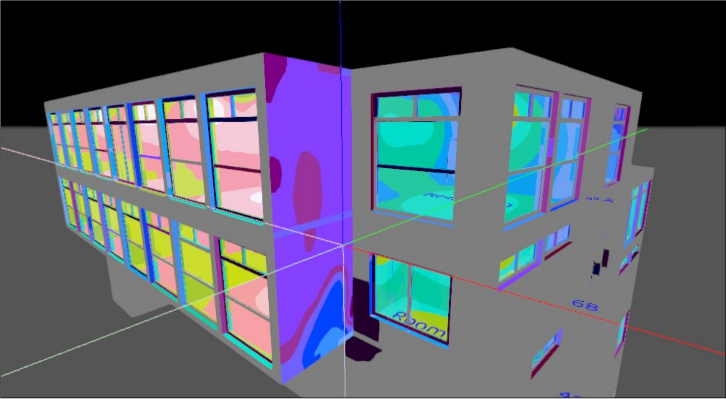
Building 1 (2), Illuminance values in [lx]
