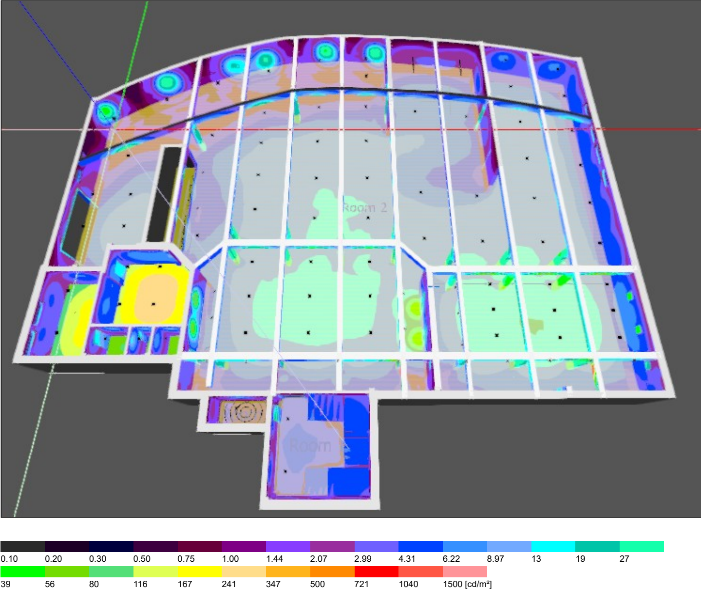
basement, Luminance values in [cd/m²]
