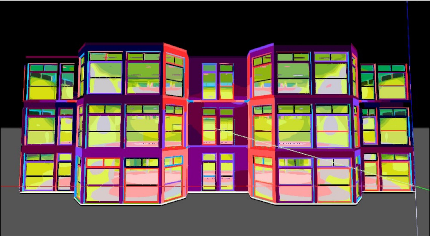
Building 1, Illuminance values in [lx]
