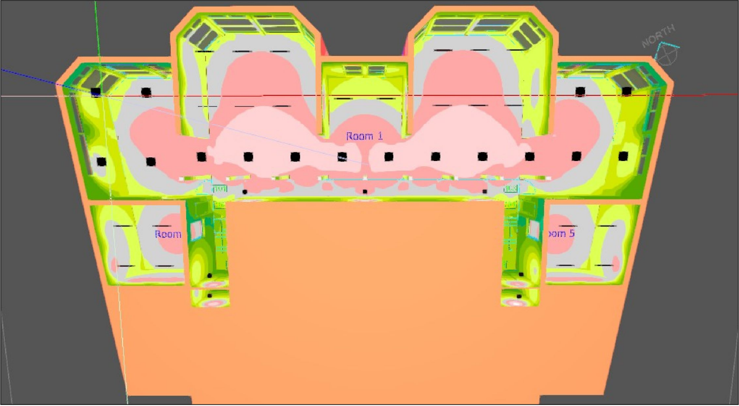
Storey 1 (3D), Illuminance values in [lx]
