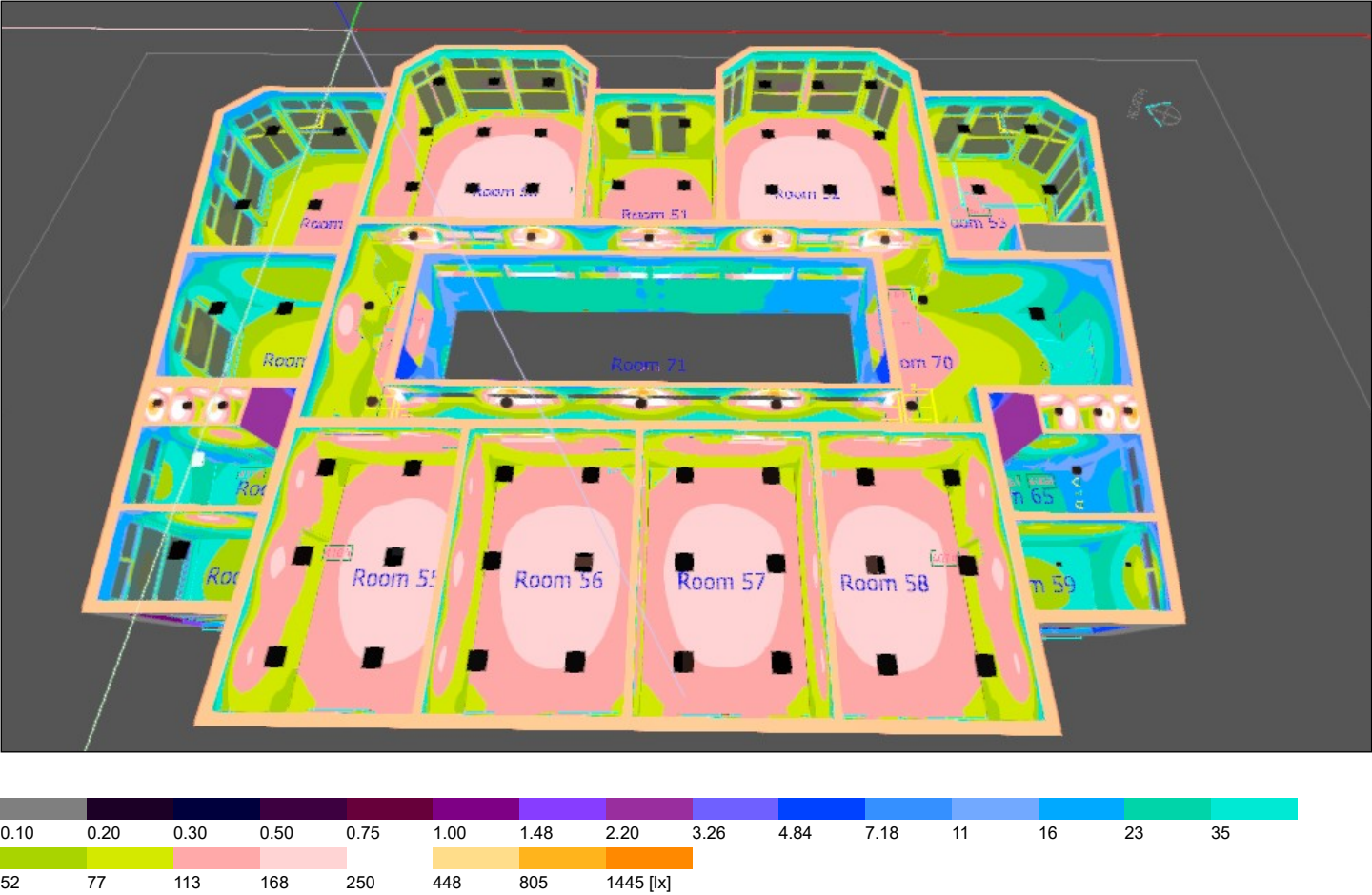
Storey 4 (3D), Illuminance values in [lx]
