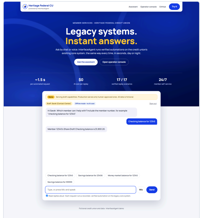
Staff mode: the employee names the member; follow-ups reuse it.
